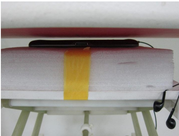
Bottom Face with Phantom 0.4 cm Gap for Earphone
