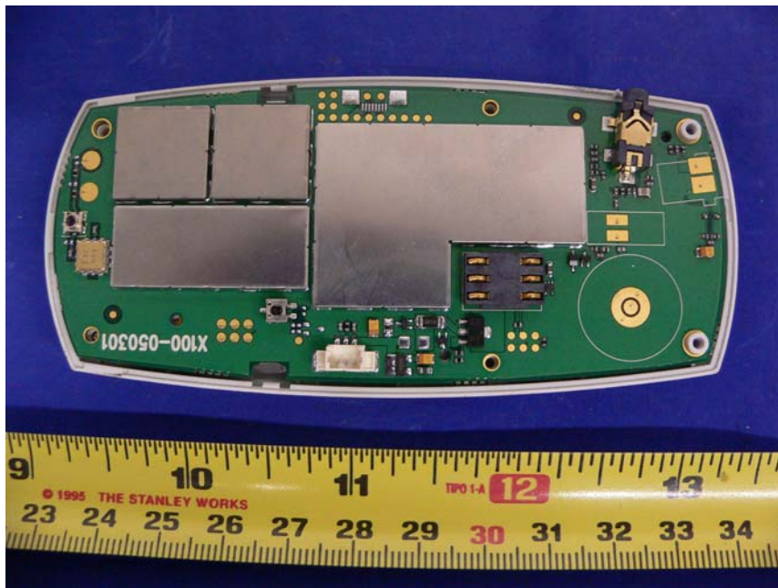
EUT - Cover Off
