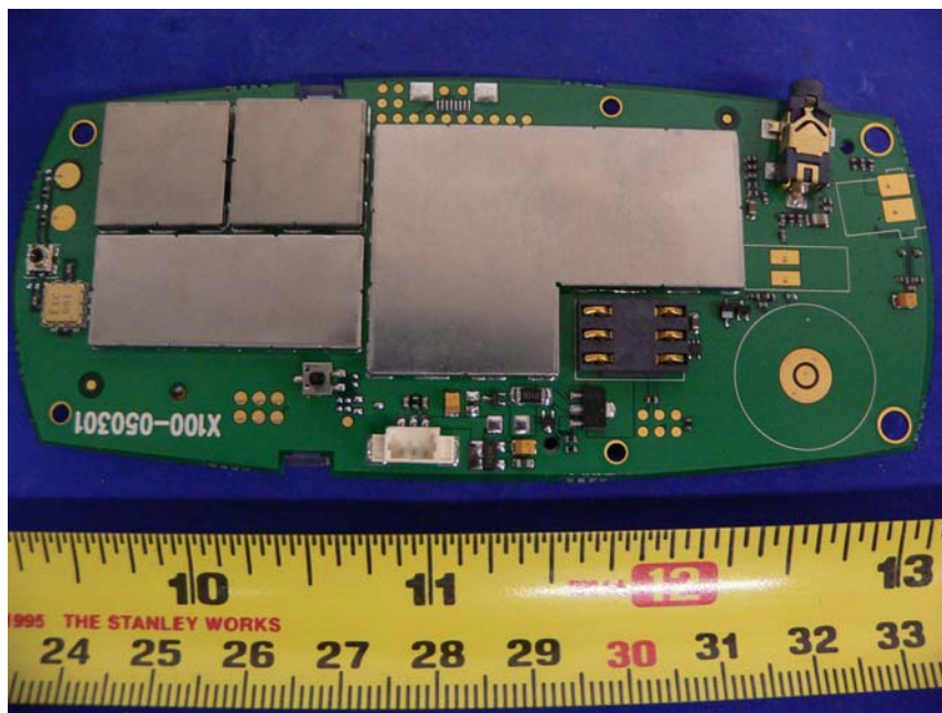
Components With Shielding
