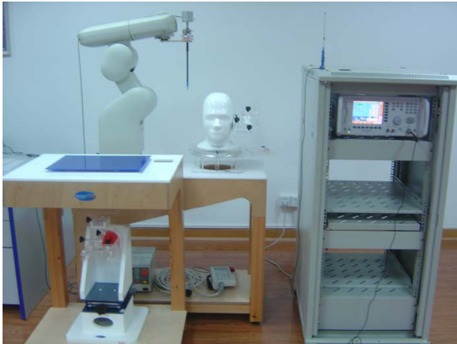
Fig.1 SARA2 System Test Layout
