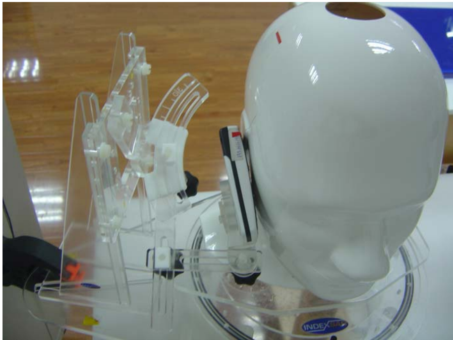
Fig.5 EUT Right Head Touch Cheek Position
