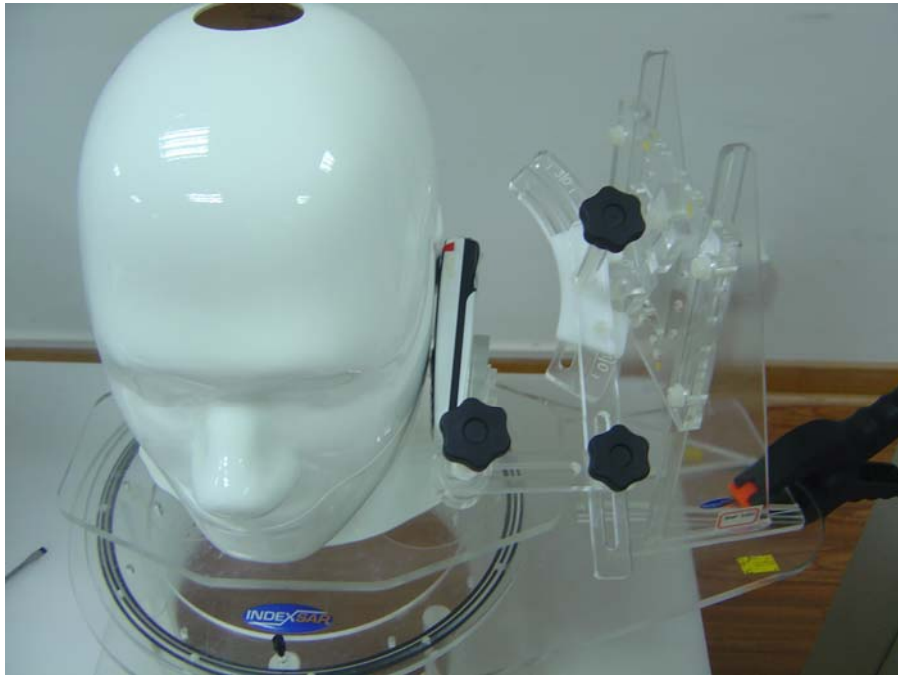
Fig.3 EUT Left Head Touch Cheek Position
