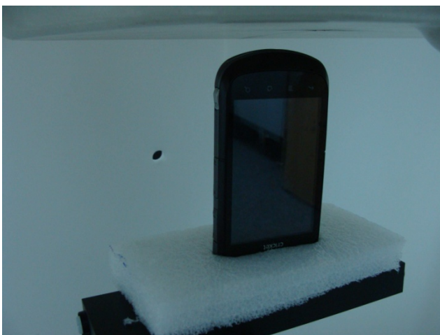
Bottom Side of DUT with Phantom 1 cm Gap
