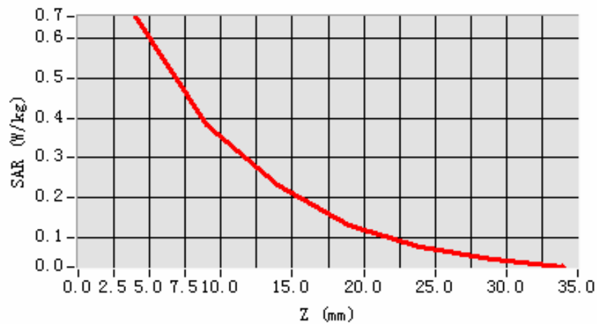
SAR, Z Axis Scan (X = -56, Y = -45)
