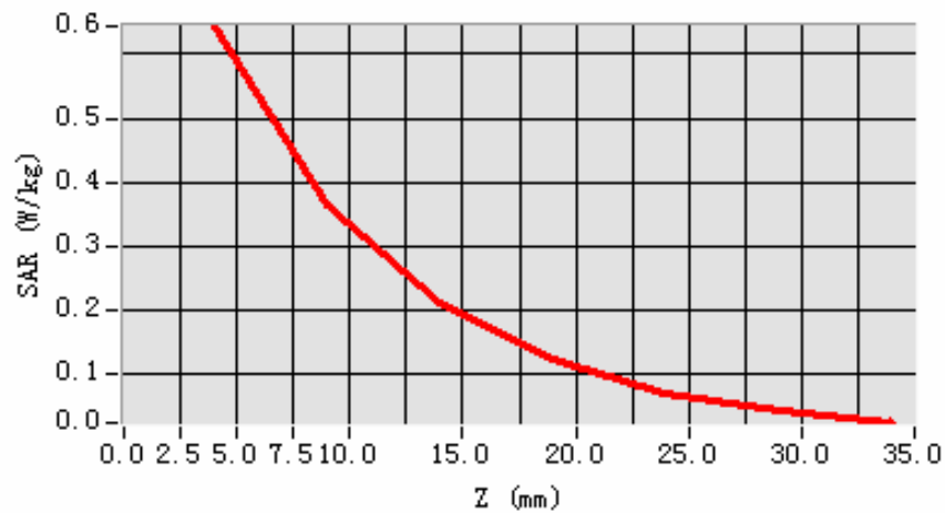
SAR, Z Axis Scan (X = -8, Y = -30)
