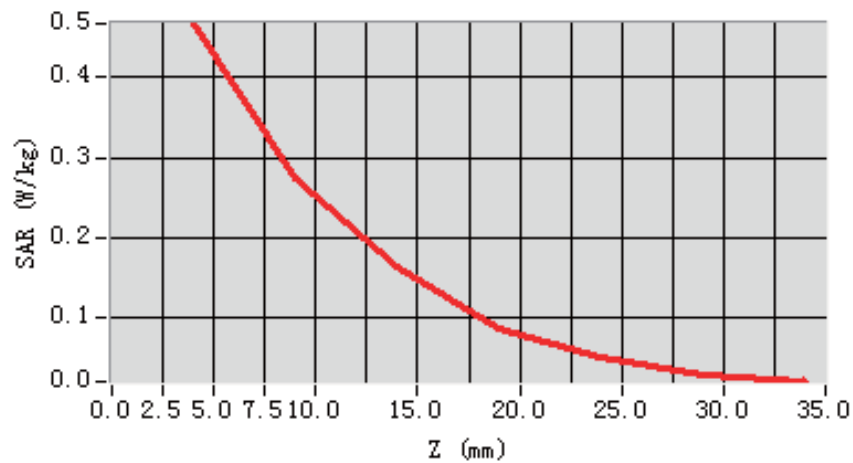
SAR, Z Axis Scan (X = -14, Y = -19)
