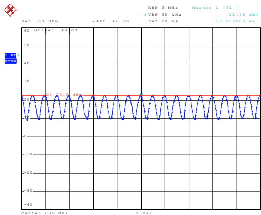
835MHz - 80% AM
