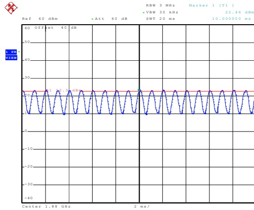
1880MHz - 80% AM
