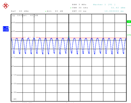
835MHz - 80% AM
