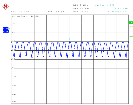
1880MHz - 80% AM
