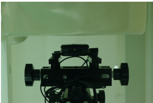
Front of the DUT with Phantom 1.5cm Gap (w/ headset)
