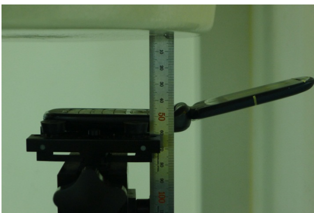
Left Cheek position - Separation distance 5cm between mouth and antenna
