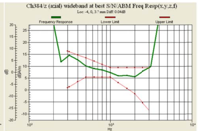
Fig. 8.2 CDMA2000 BC0 Ch384
