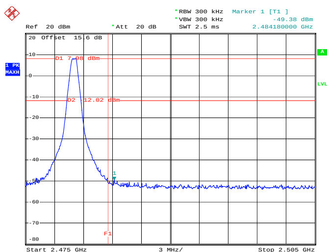
High Band Edge Plot on Channel 78
