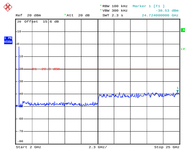
Conducted Spurious Emission Plot on Bluetooth LE GFSK Channel 00
