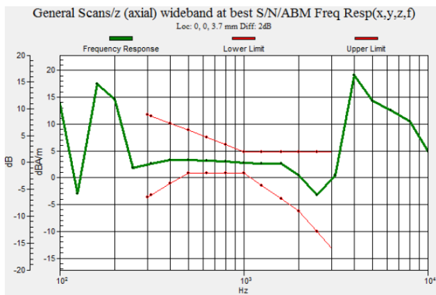
Fig 8.3 GSM850 Ch251
