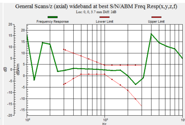
Fig 8.4 GSM1900 Ch512
