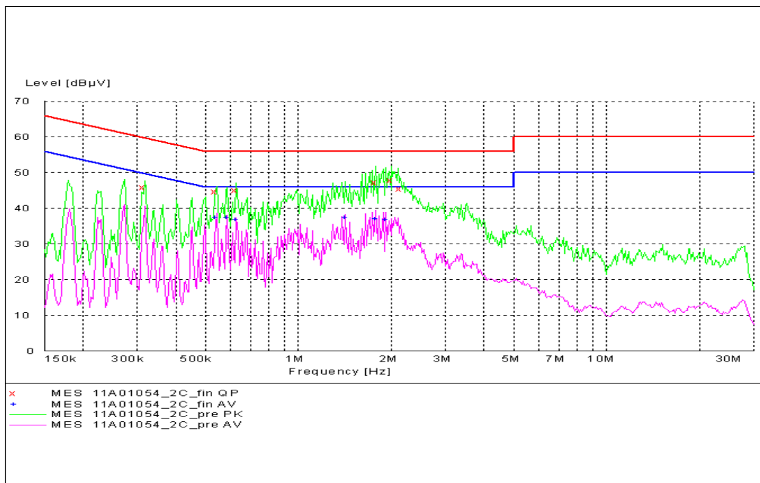
Figure A.6 Conducted Emission
