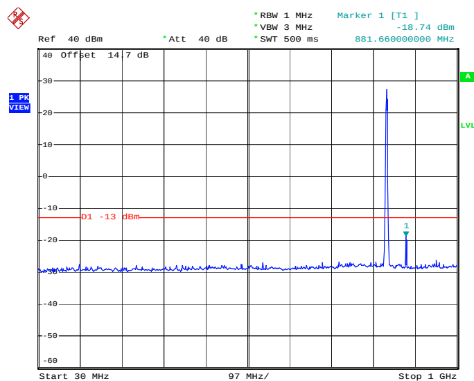
Conducted Emission Plot between 30MHz ~ 1GHz
