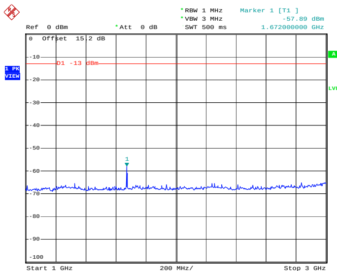
Conducted Emission Plot between 1GHz ~ 3GHz
