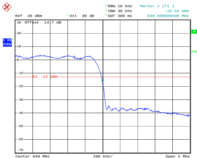
Higher Band Edge Plot on Channel 777
