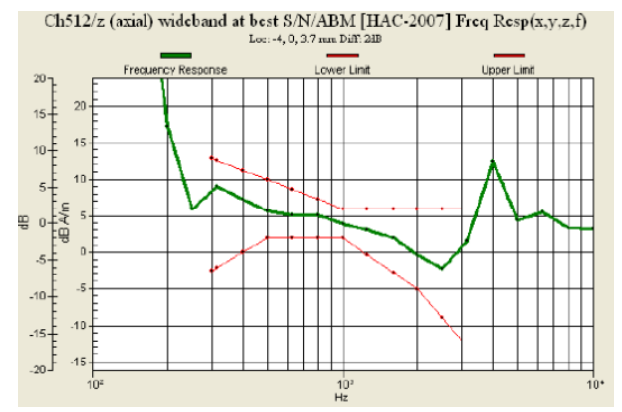
Fig. 9.4 GSM1900 Ch512
