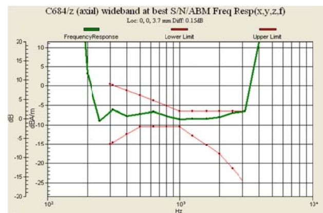
Fig 8.6 CDMA2000 BC10 Ch684
