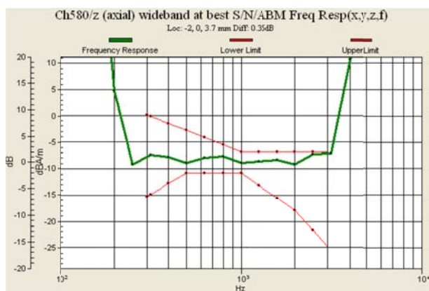
Fig 8.5 CDMA2000 BC10 Ch580
