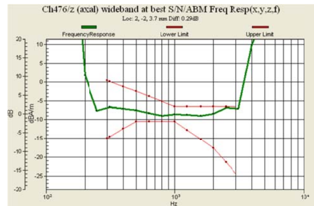
Fig 8.4 CDMA2000 BC10 Ch476
