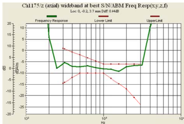
Fig 8.3 CDMA2000 BC1 Ch1175
