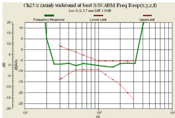
Fig 8.1 CDMA2000 BC1 Ch25
