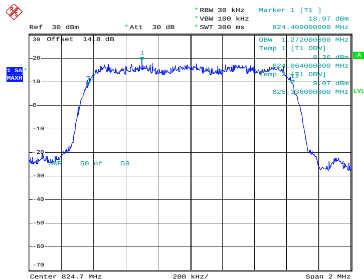
99% Occupied Bandwidth Plot on Channel 1013 (824.7 MHz)
