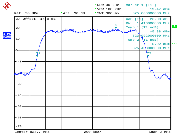
26dB Bandwidth Plot on Channel 1013 (824.7 MHz)
