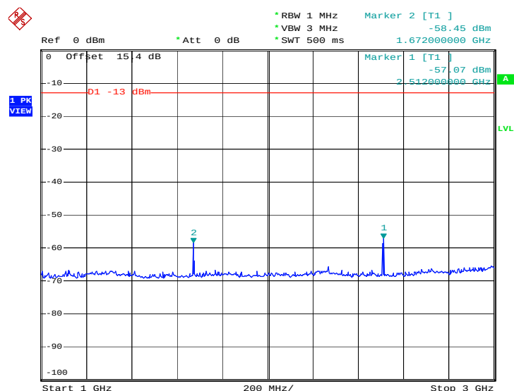
Conducted Spurious Emission Plot between 1GHz ~ 3GHz
