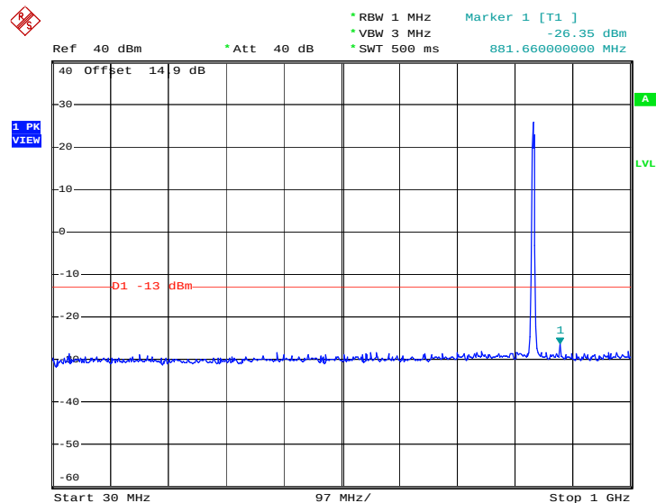
Conducted Spurious Emission Plot between 30MHz ~ 1GHz
