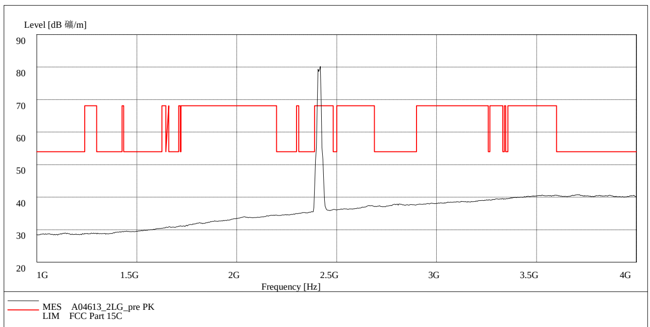
Fig. 56 Radiated Spurious Emission (802.11g, Ch1, 1 GHz-4 GHz)
