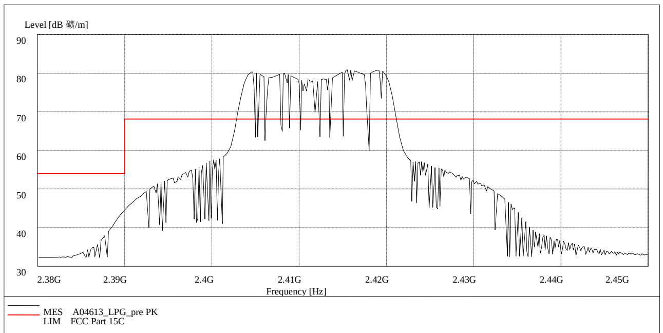
Fig. 54 Radiated Spurious Emission (Power): 802.11g, ch1, 2.38 GHz - 2.45GHz
