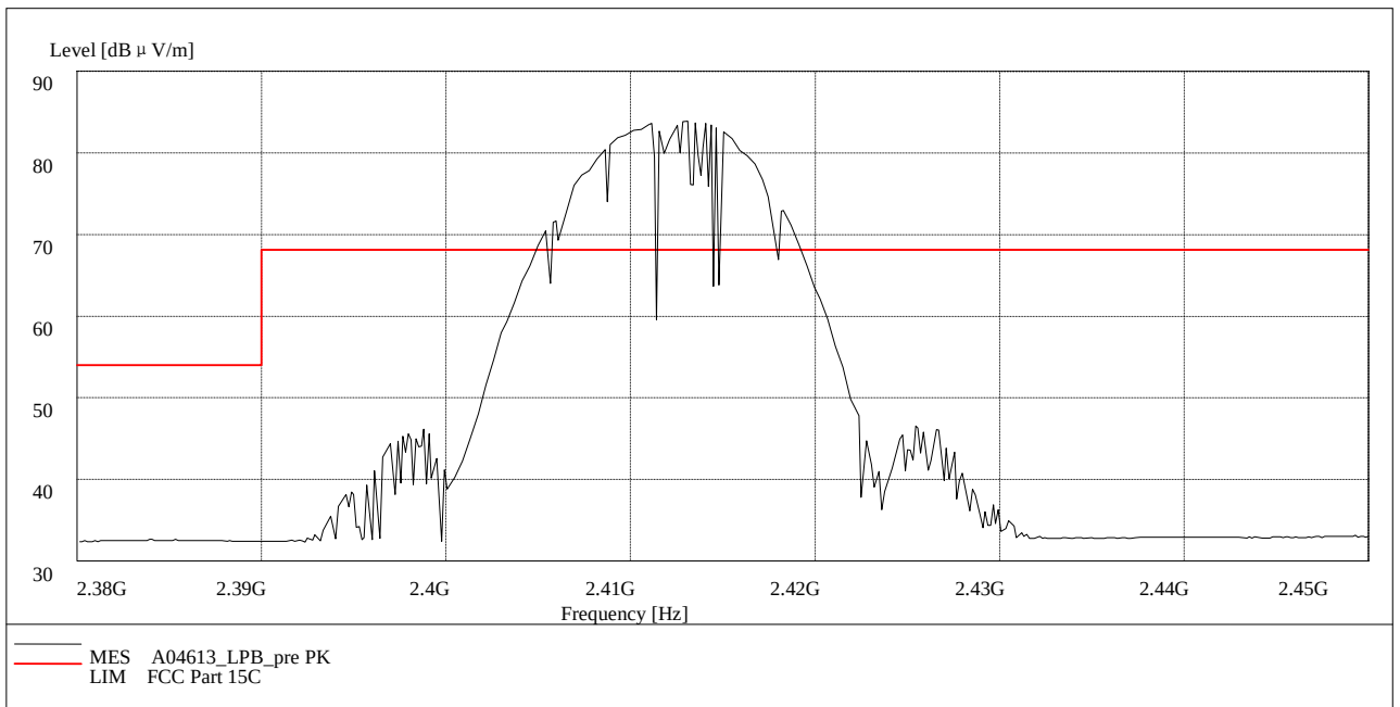
Fig. 43 Radiated Spurious Emission (Power): 802.11b, ch1, 2.38 GHz - 2.45GHz
