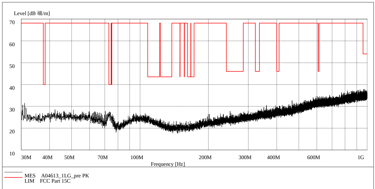
Fig. 55 Radiated Spurious Emission (802.11g, Ch1, 30 MHz-1 GHz)
