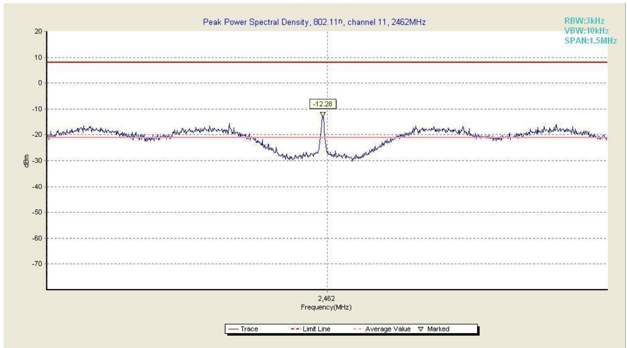
Fig. 9 Power Spectral Density (802.11-20MHz, Ch 11)
