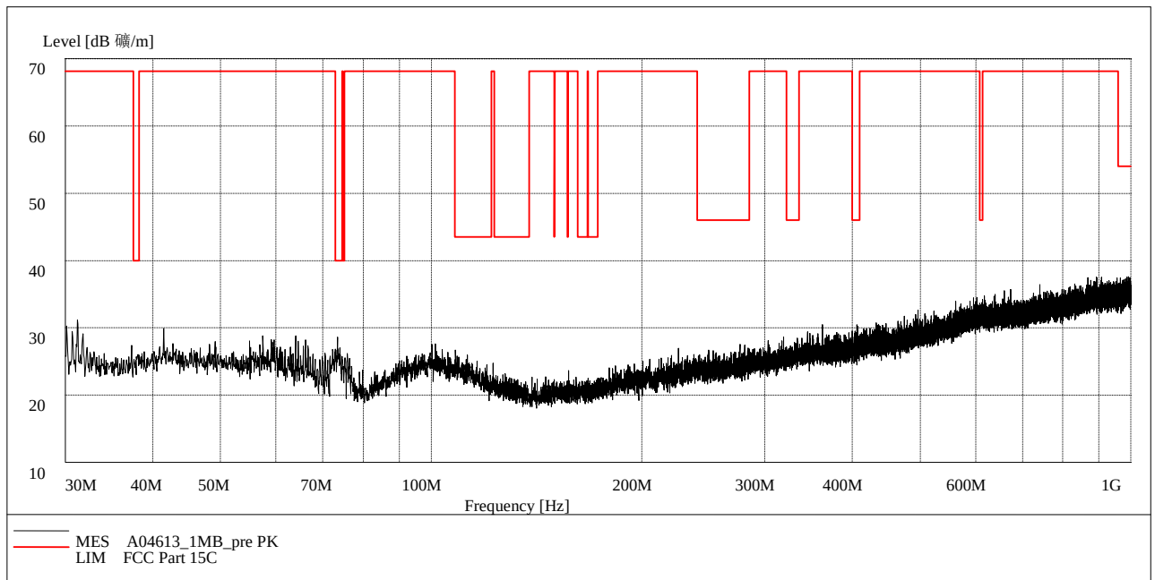
Fig. 47 Radiated Spurious Emission (802.11b, Ch6, 30 MHz-1 GHz)
