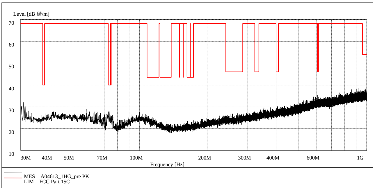
Fig. 62 Radiated Spurious Emission (802.11g, Ch11, 30 MHz-1 GHz)
