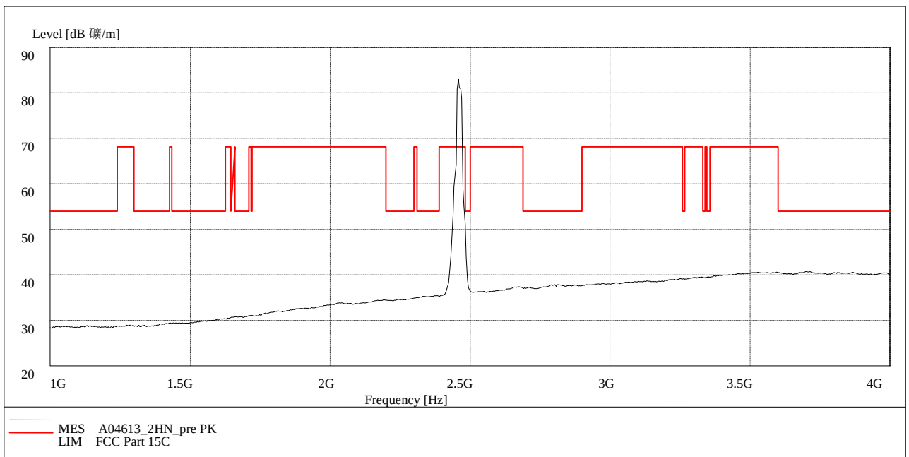
Fig. 74 Radiated Spurious Emission (802.11n-20MHz, Ch11, 1 GHz-4 GHz)
