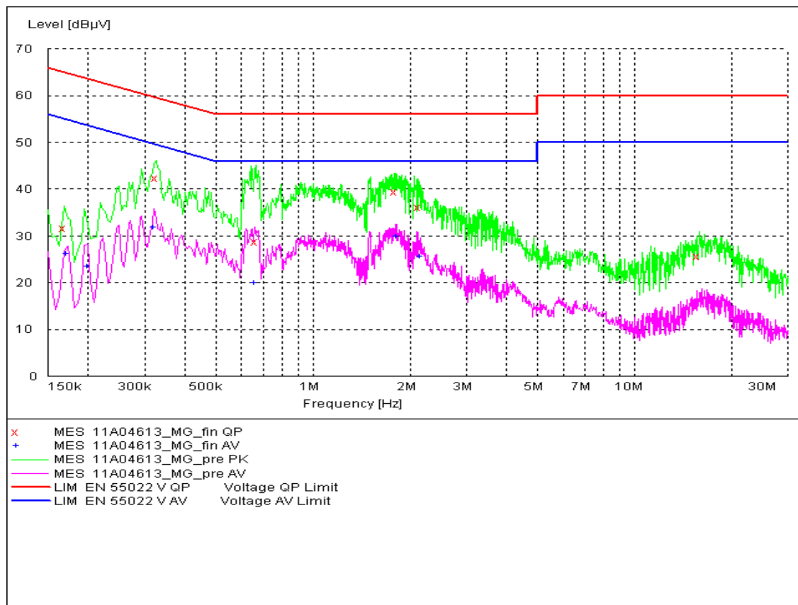
Fig. 78 AC Powerline Conducted Emission-802.11g
