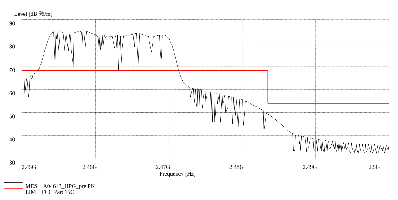
Fig. 61 Radiated Spurious Emission (Power): 802.11g, ch11, 2.45 GHz - 2.50GHz
