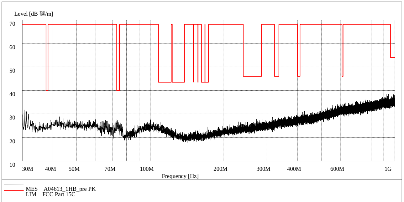
Fig. 51 Radiated Spurious Emission (802.11b, Ch11, 30 MHz-1 GHz)
