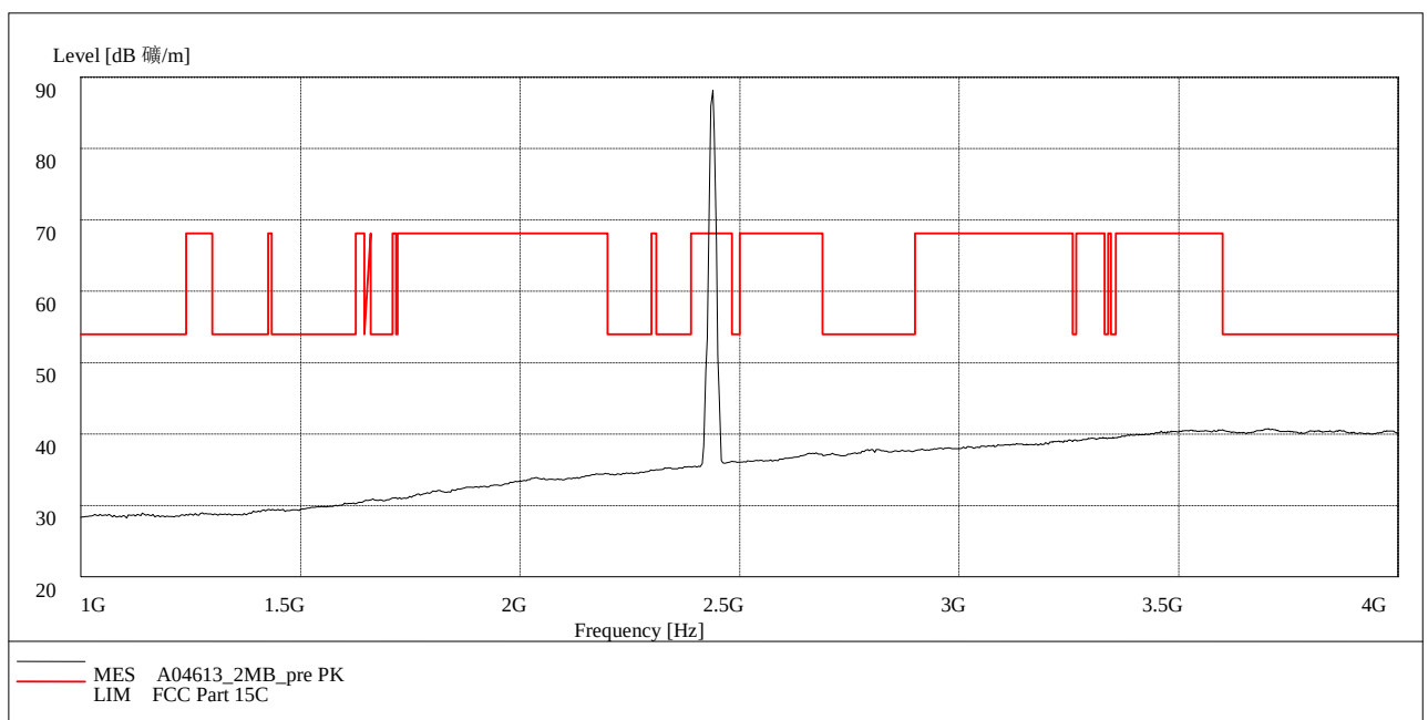
Fig. 48 Radiated Spurious Emission (802.11b, Ch6, 1 GHz-4 GHz)
