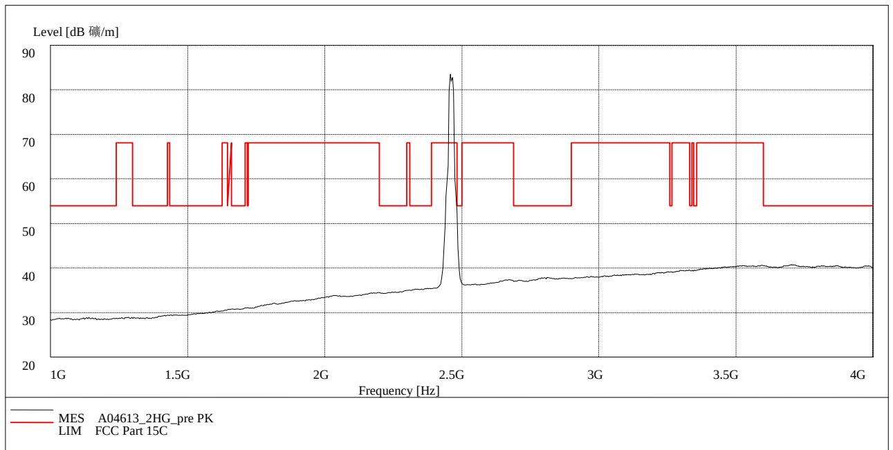
Fig. 63 Radiated Spurious Emission (802.11g, Ch11, 1 GHz-4 GHz)
