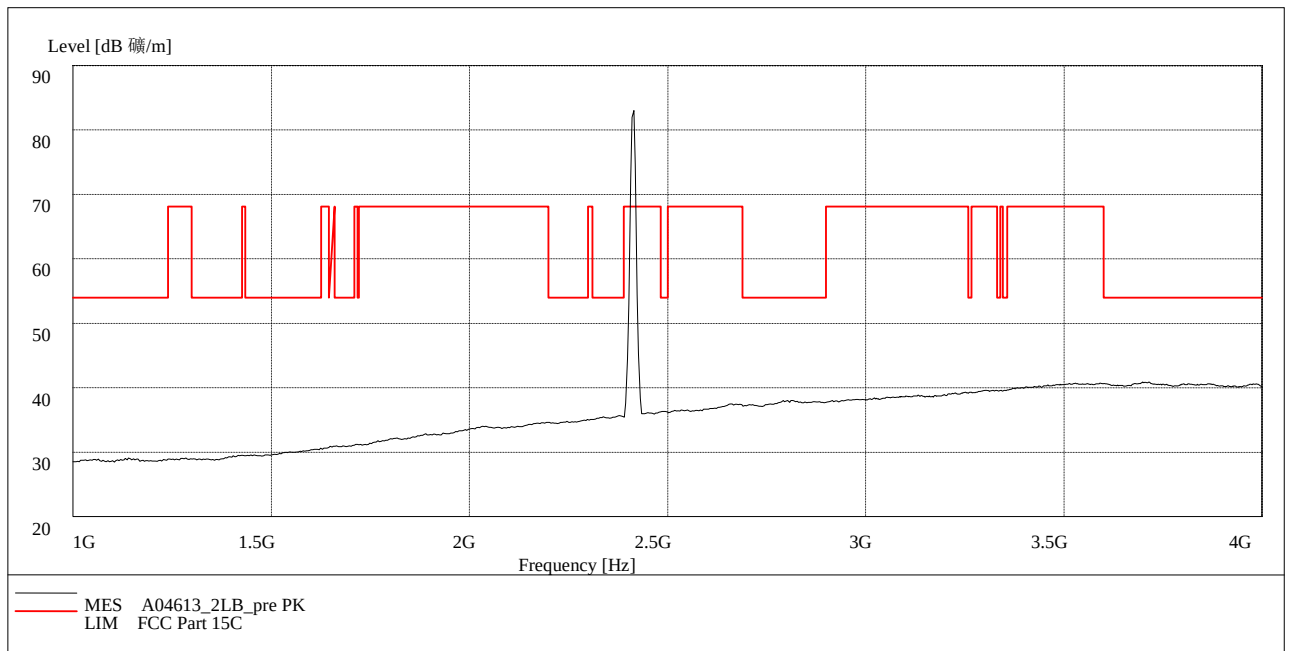
Fig. 45 Radiated Spurious Emission (802.11b, Ch1, 1 GHz-4 GHz)
