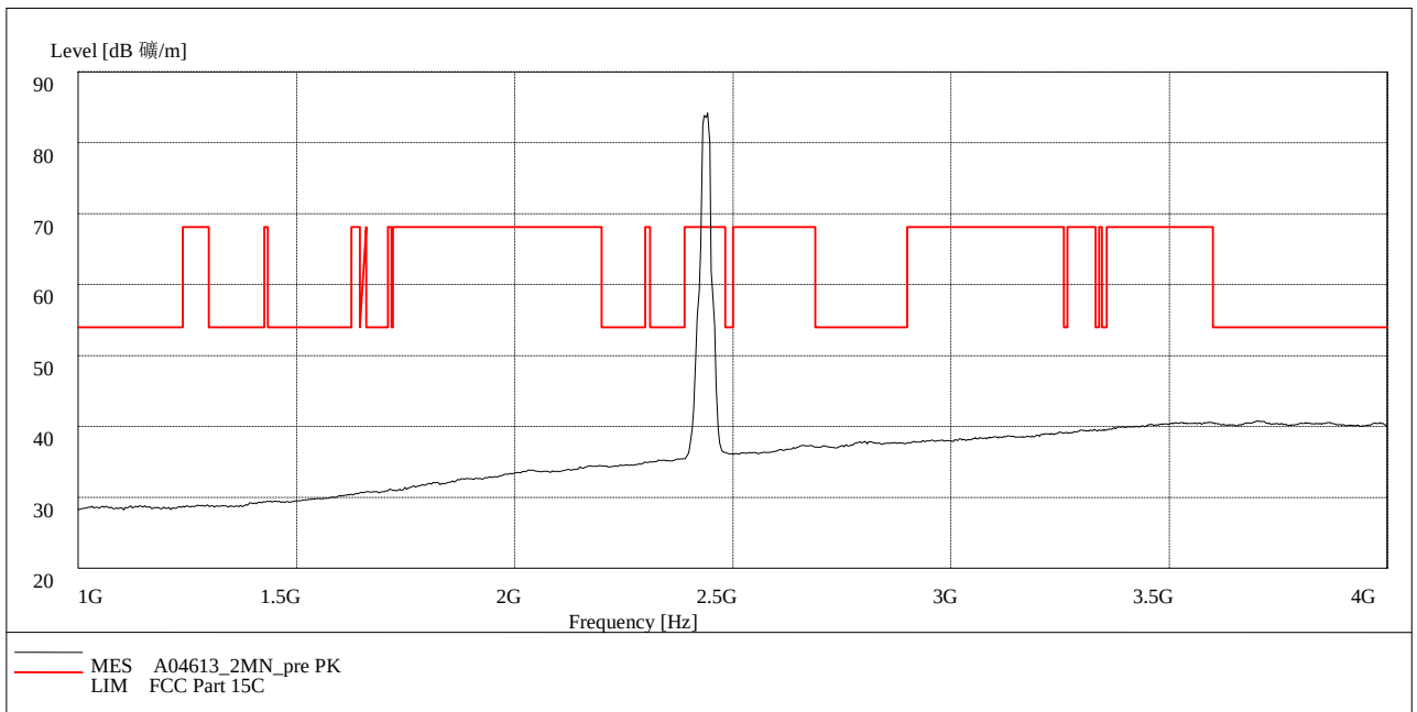
Fig. 70 Radiated Spurious Emission (802.11n-20MHz, Ch6, 1 GHz-4 GHz)
