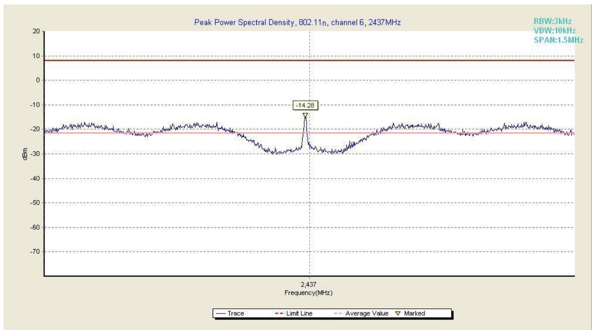
Fig. 8 Power Spectral Density (802.11-20MHz, Ch 6)
