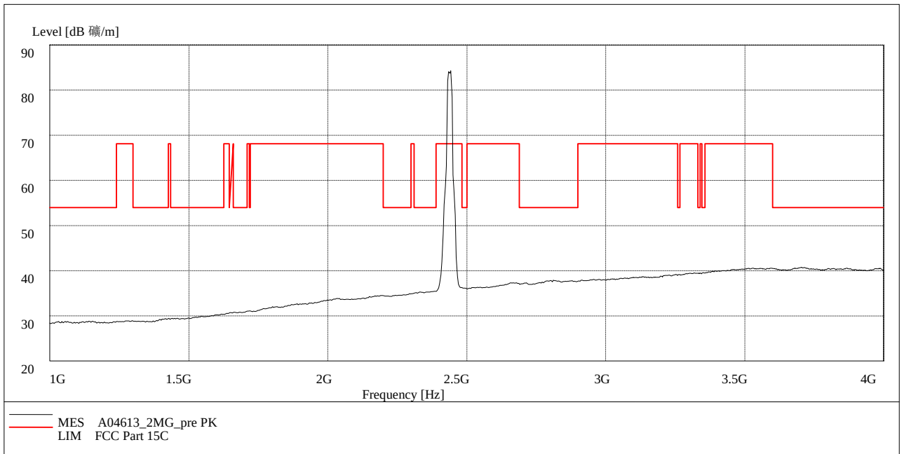
Fig. 59 Radiated Spurious Emission (802.11g, Ch6, 1 GHz-4 GHz)
