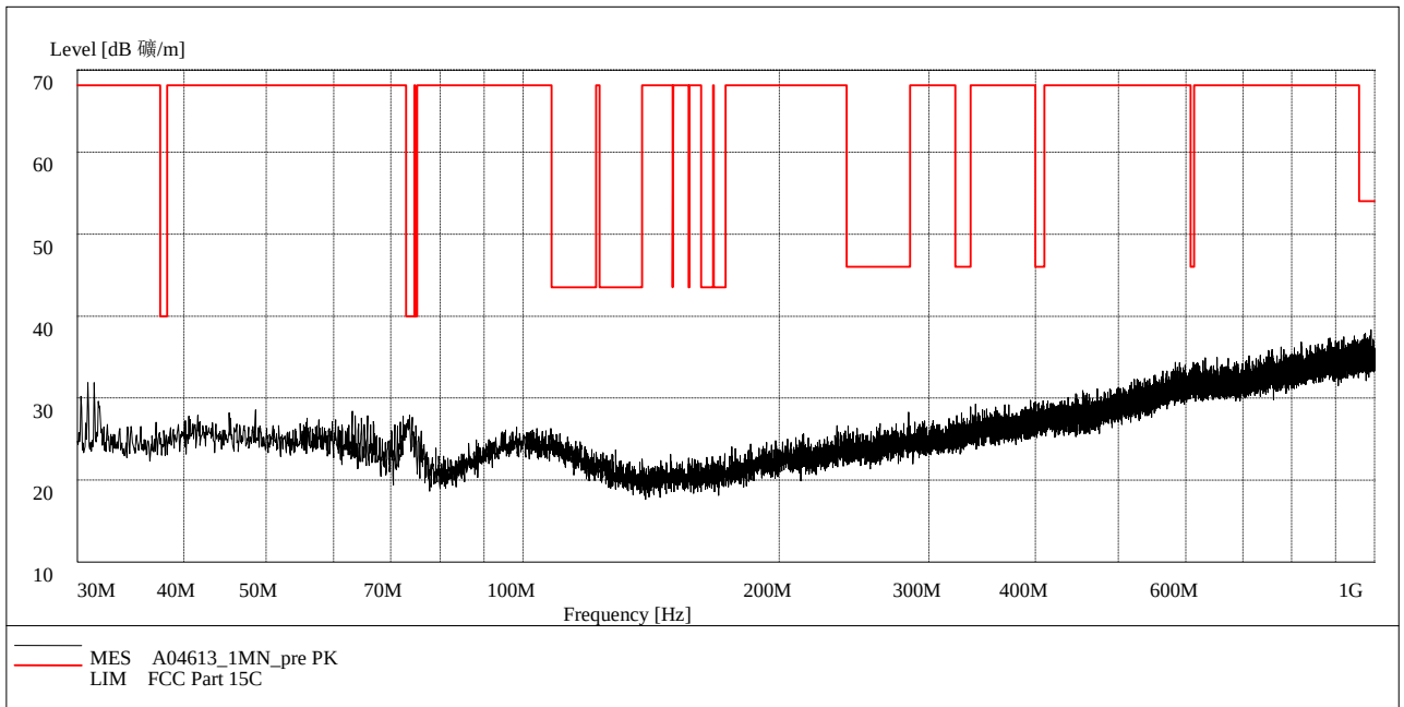
Fig. 69 Radiated Spurious Emission (802.11n-20MHz, Ch6, 30 MHz-1 GHz)
