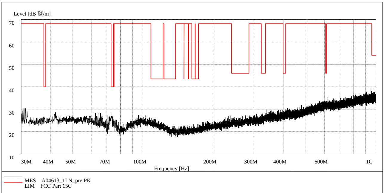
Fig. 66 Radiated Spurious Emission (802.11n-20MHz, Ch1, 30 MHz-1 GHz)
