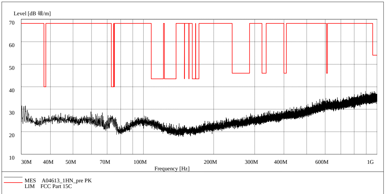
Fig. 73 Radiated Spurious Emission (802.11n-20MHz, Ch11, 30 MHz-1 GHz)
