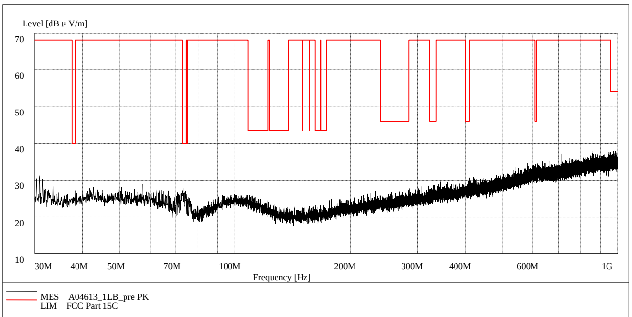
Fig. 44 Radiated Spurious Emission (802.11b, Ch1, 30 MHz-1 GHz)
