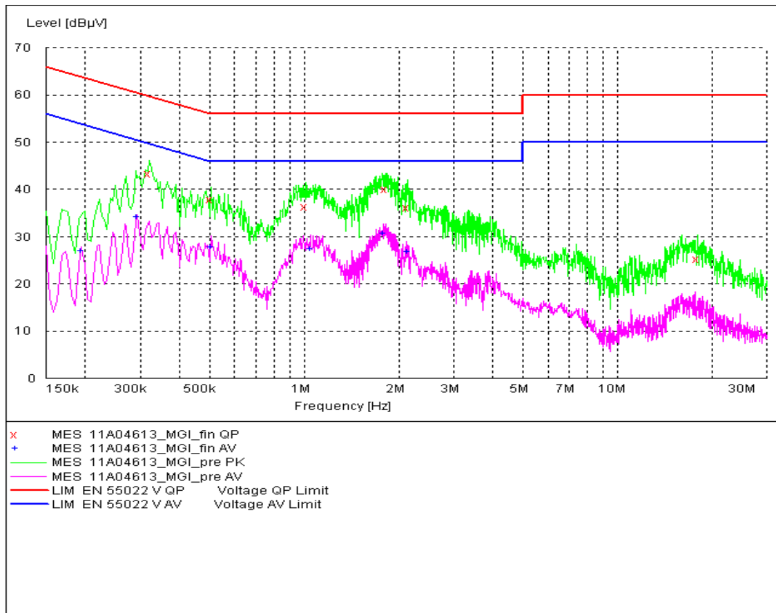
Fig. 77 AC Powerline Conducted Emission-802.11b
