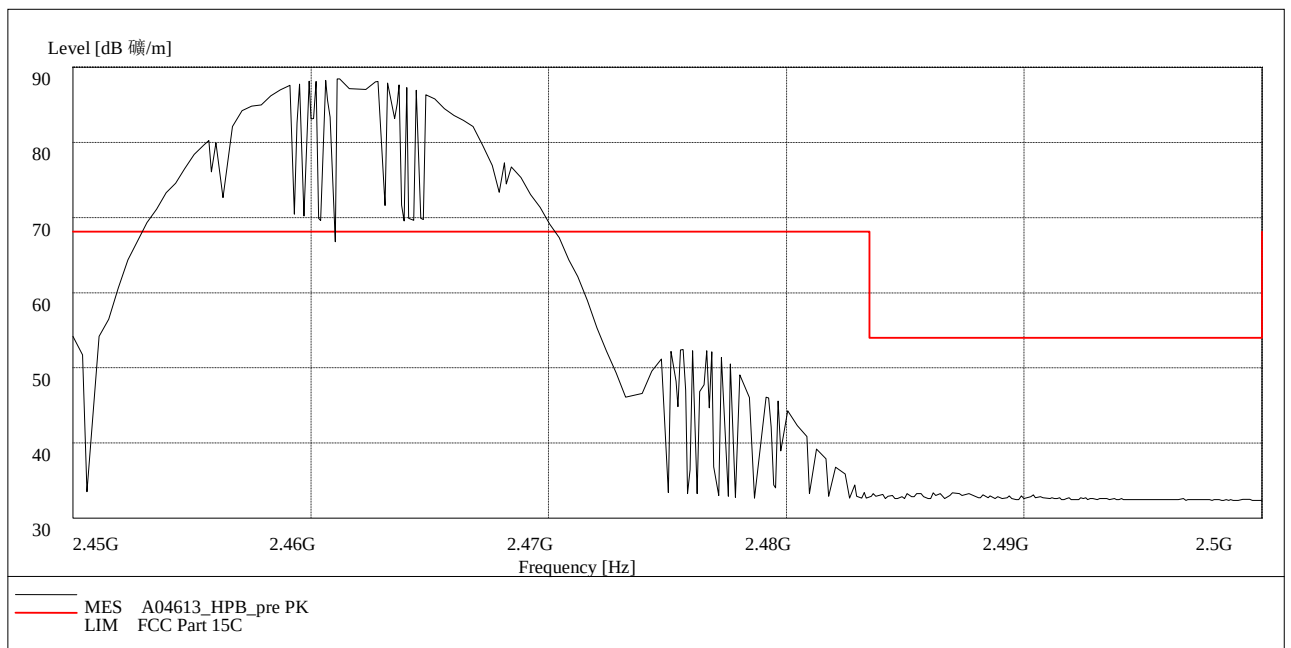
Fig. 50 Radiated Spurious Emission (Power): 802.11b, ch11, 2.45 GHz - 2.50GHz
