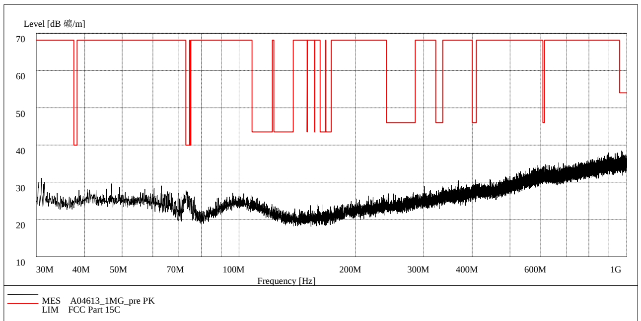
Fig. 58 Radiated Spurious Emission (802.11g, Ch6, 30 MHz-1 GHz)
