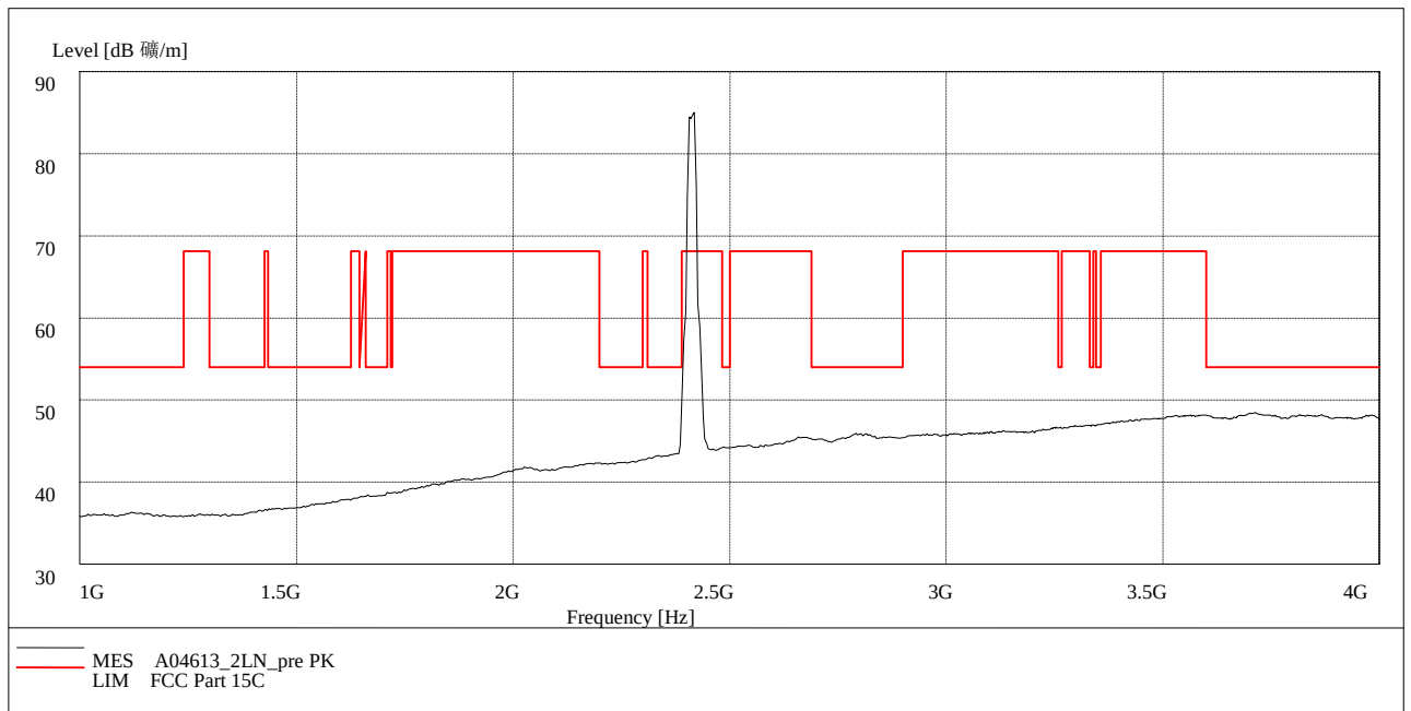
Fig. 67 Radiated Spurious Emission (802.11n-20MHz, Ch1, 1 GHz-4 GHz)
