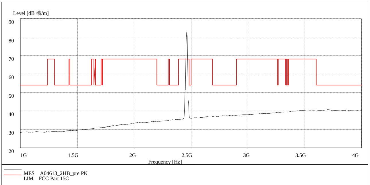
Fig. 52 Radiated Spurious Emission (802.11b, Ch11, 1 GHz-4 GHz)
