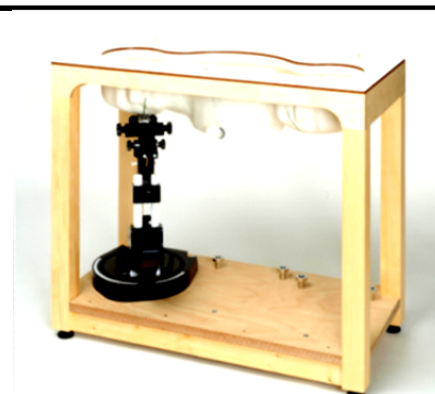
Fig 5.6 Photo of SAM Phantom
