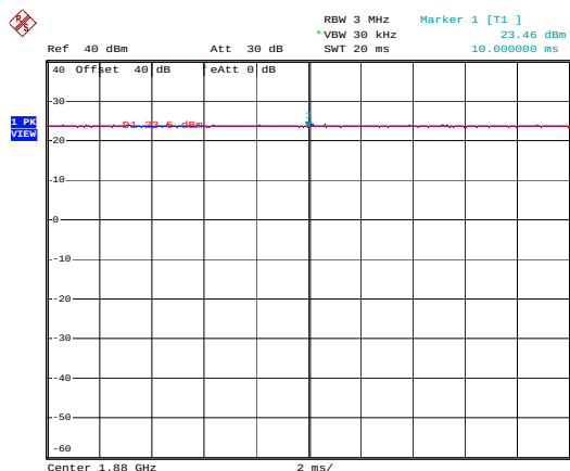
1880MHz - CDMA (Full Rate)
