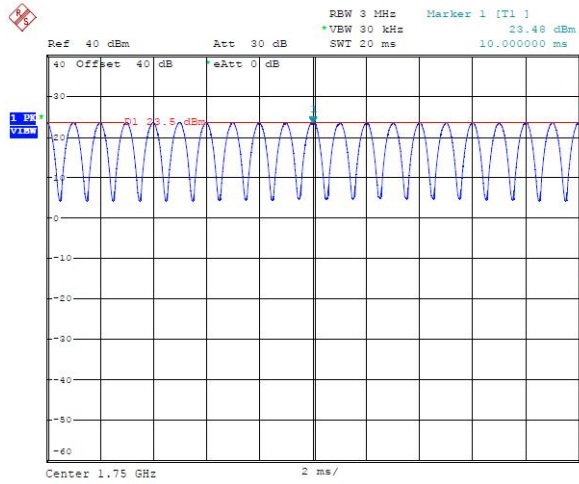
1750MHz - 80% AM
