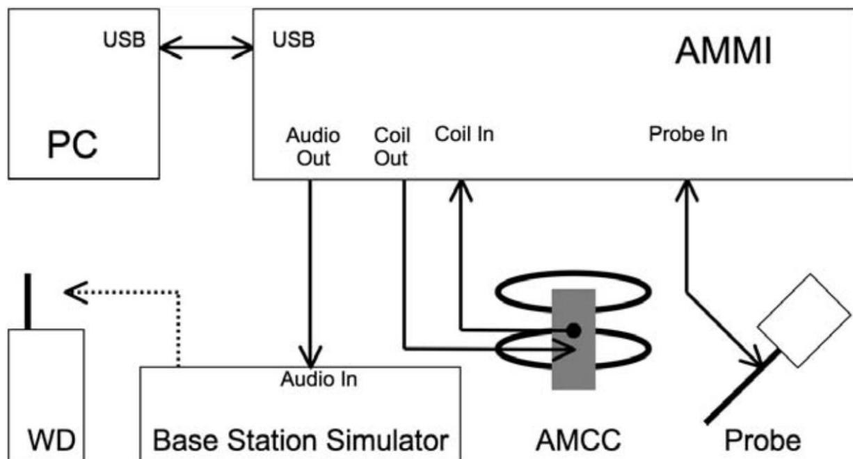
Fig. 5.10 T-Coil setup cabling
