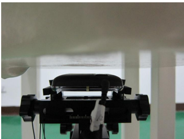
Face of the DUT with Phantom 1.0 cm Gap (Headset)
