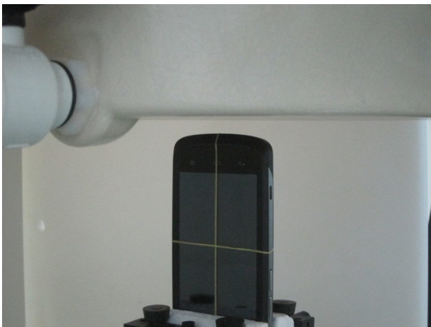
Bottom Side of the EUT with Phantom 1.0 cm Gap
