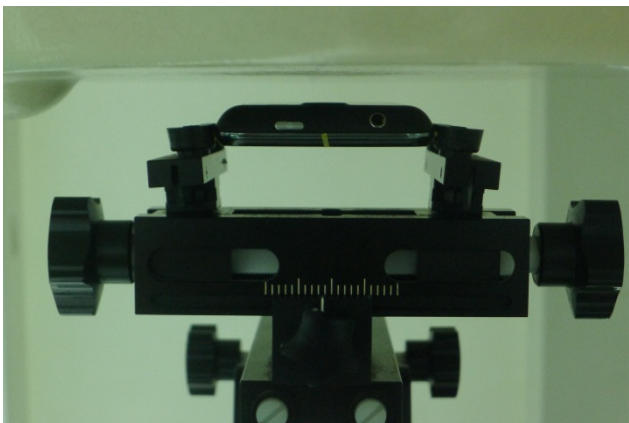
Back of the EUT with Phantom 1.0 cm Gap
