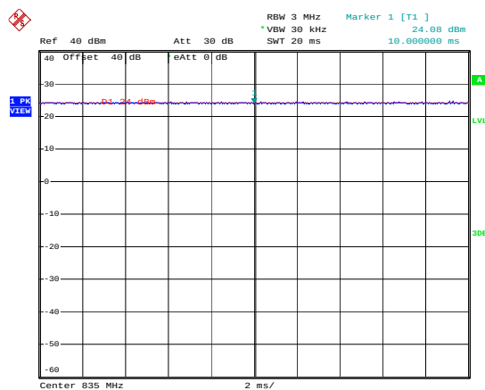
835MHz - CDMA (Full Rate)
