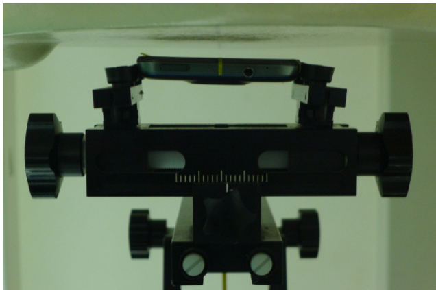
Front of the DUT with Phantom 1 cm Gap
