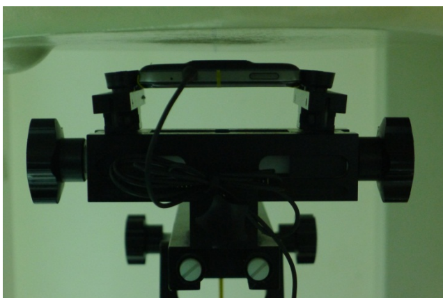
Back of the DUT with Phantom 1 cm Gap with headset
