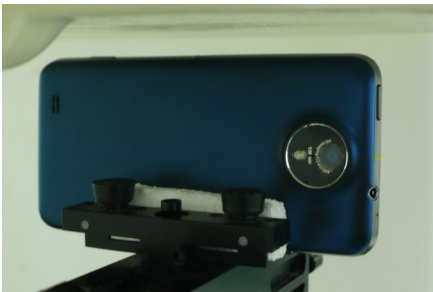
Right Side of the DUT with Phantom 1 cm Gap
