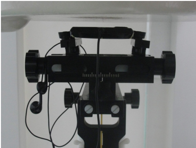
Rear Face with Earphone of the DUT with Phantom 1 cm Gap
