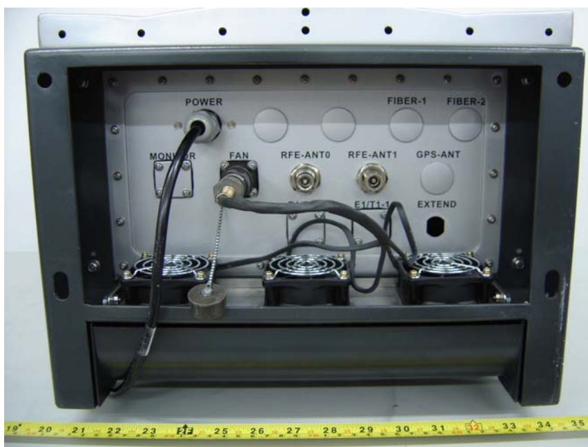
EUT-Bottom View
