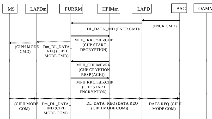
FIGURE 39 ENCRYPTION
