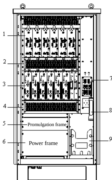
FIGURE 4 LAYOUT OF THE ZXG10 OB06 SYSTEM
