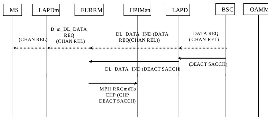
FIGURE 40 SACCH DEACTIVATION
