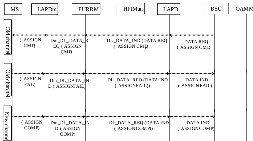
FIGURE 38 CONNECTION ALLOCATION
