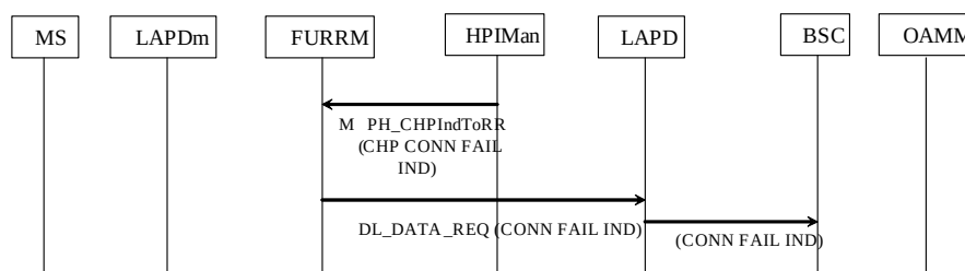
FIGURE 59 CONNECTION FAILURE
