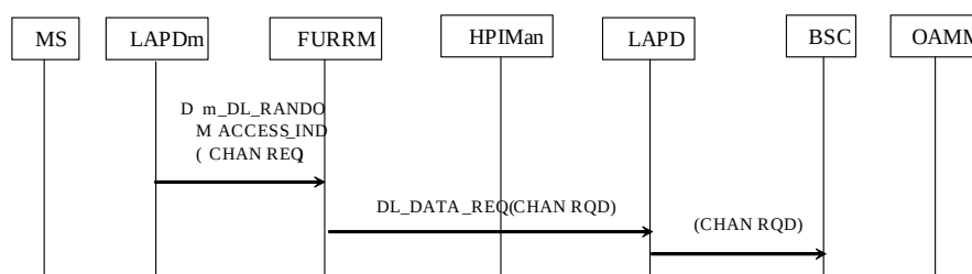
FIGURE 48 ACCESS REQUEST
