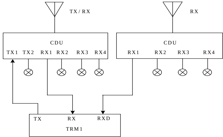
FIGURE 74 LOGICAL CONNECTION RELATIONSHIP BETWEEN THE COMBINER UNITS AND DISTRIBUTION UNITS OF THE O1-TYPE SITE
