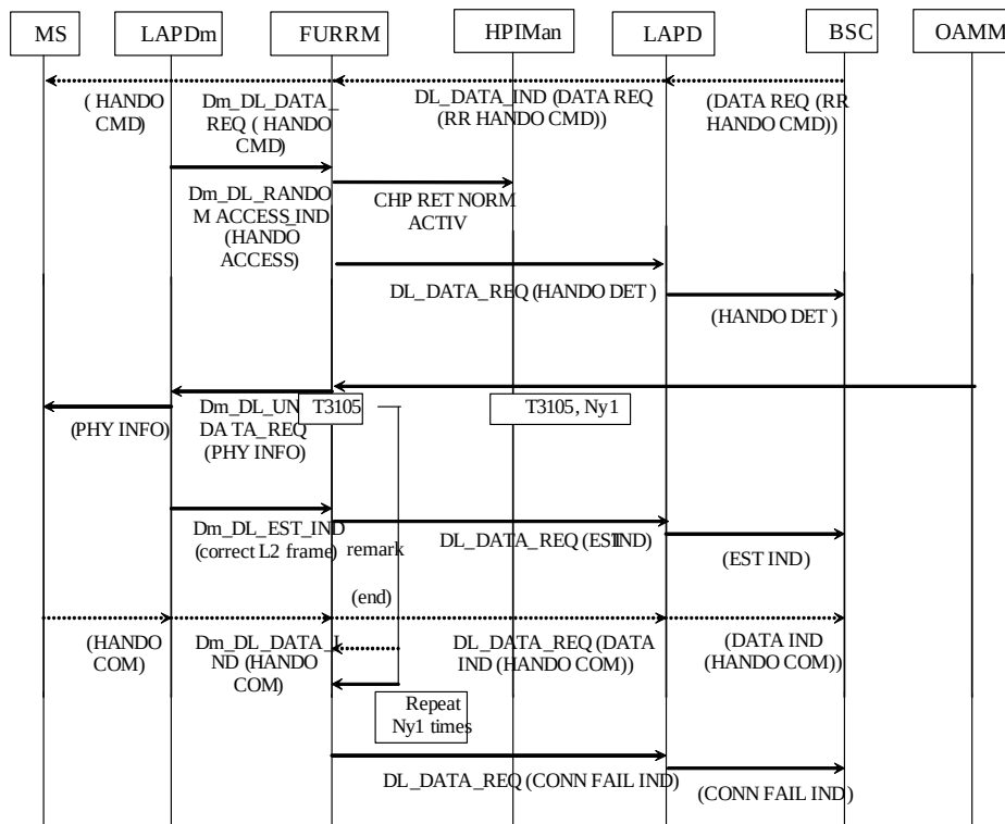
FIGURE 35 HANDOVER
