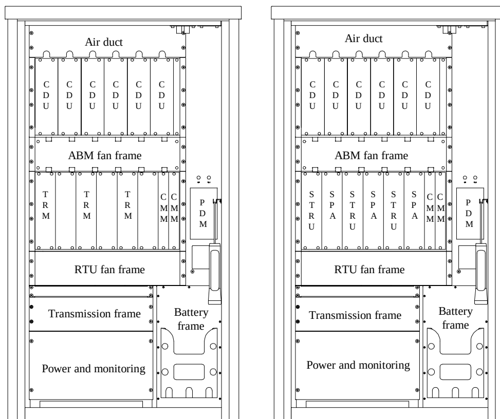
FIGURE 83 CONFIGURATION OF S1/1/1-TYPE SITES
