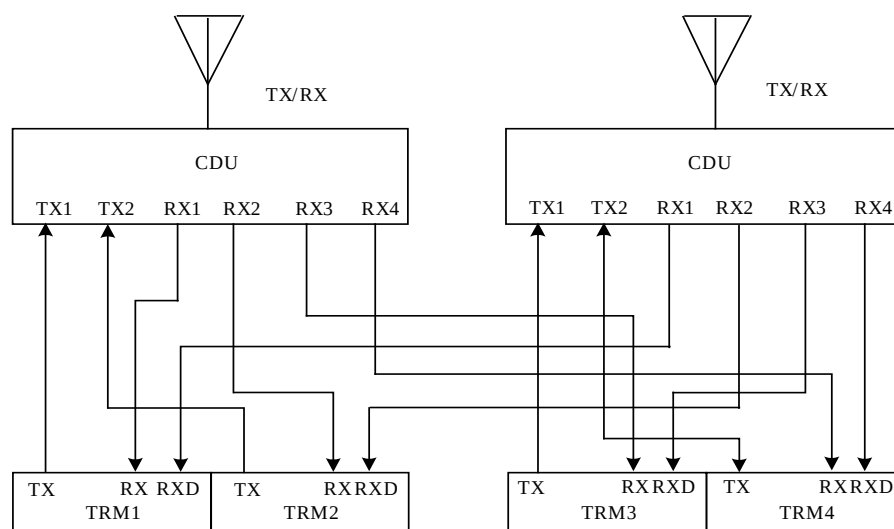
FIGURE 80 LOGICAL CONNECTION RELATIONSHIP BETWEEN THE COMBINER UNITS AND DISTRIBUTION UNITS OF O4-TYPE SITES
