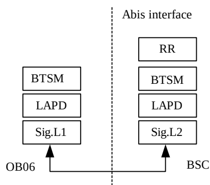
FIGURE 10 CIRCUIT SERVICE PROTOCOL LAYERED STRUCTURE OF ABIS INTERFACE
