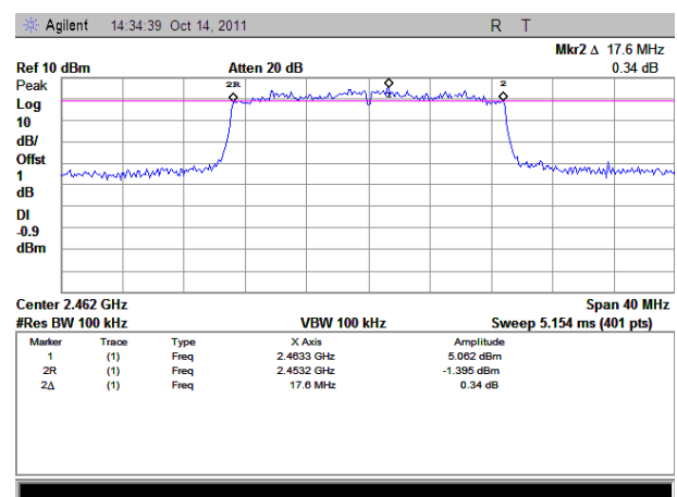
(Plot F: Chain2_Channel 11: 2462MHz)
