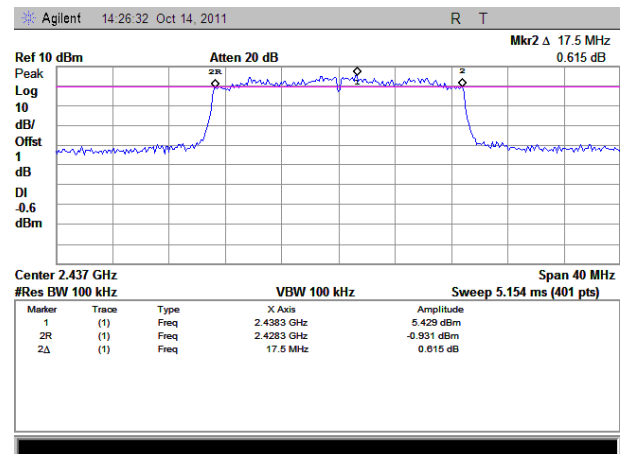
(Plot D: Chain2_Channel 6: 2437 MHz)
