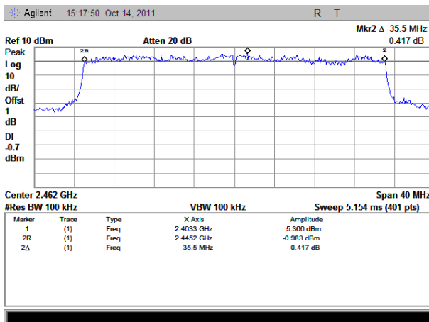
(Plot E: Chain1_Channel 9: 2462MHz)
