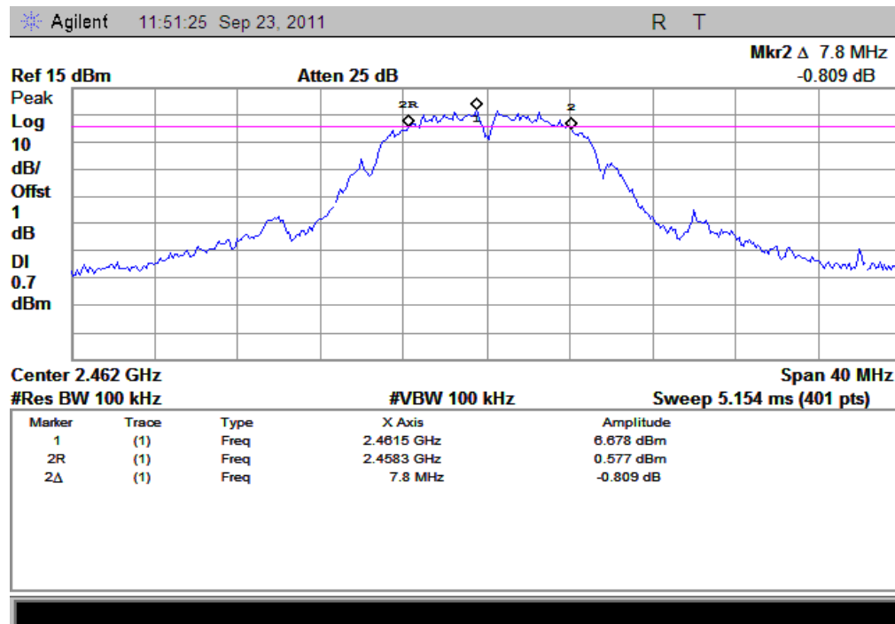
(Plot C: Channel 11: 2462MHz)
