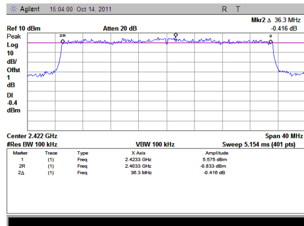
(Plot B: Chain2_Channel 3: 2422MHz)
