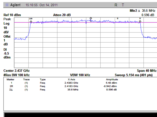
(Plot D: Chain2_Channel 6: 2437 MHz)
