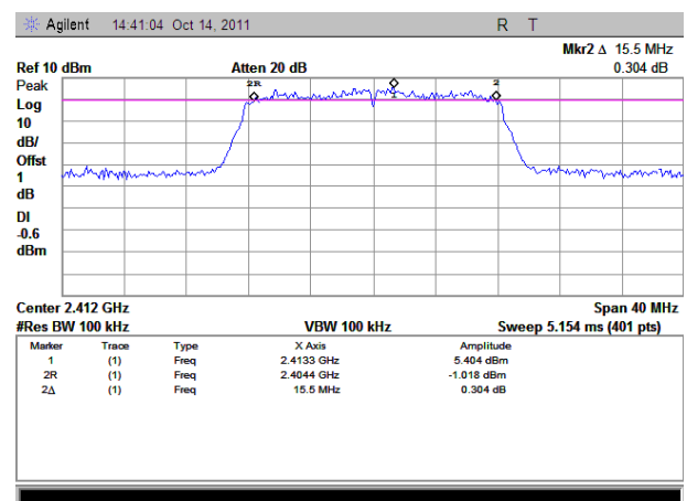
(Plot B: Chain2_Channel 1: 2412MHz)
