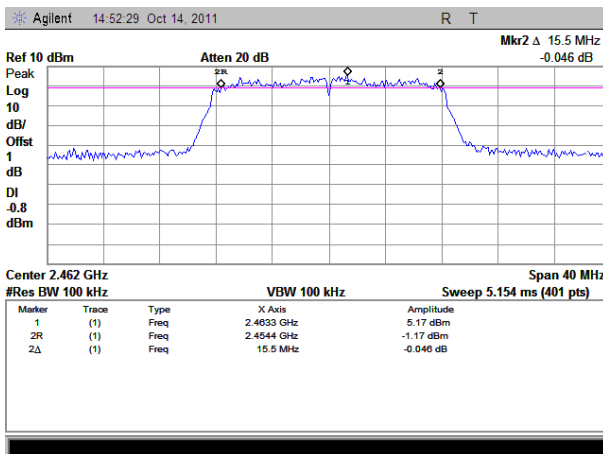
(Plot E: Chain1_Channel 11: 2462MHz)
