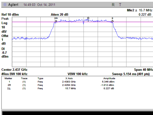
(Plot C: Chain1_Channel 6: 2437 MHz)
