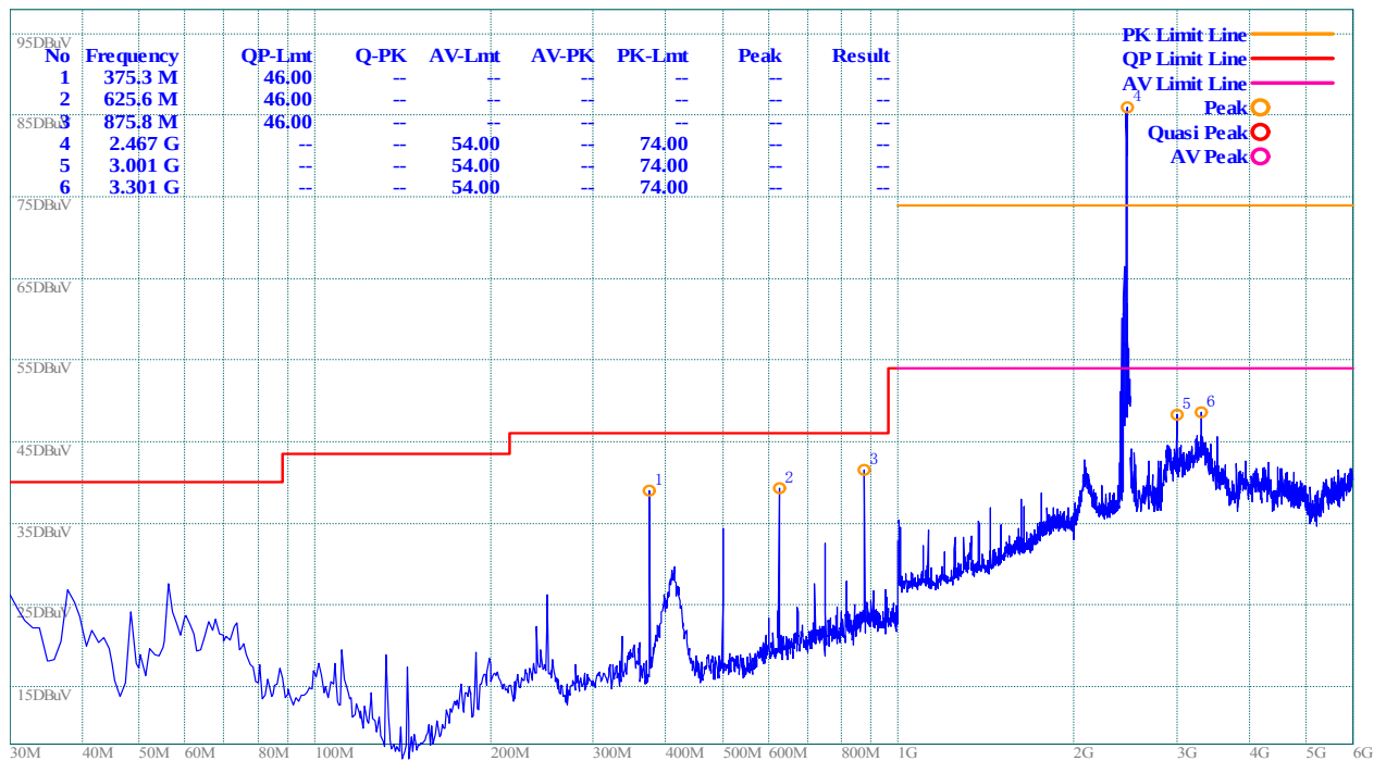
(Plot C: 30M – 6G, Test Antenna Horizontal)
