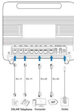
Figure 4 Cable Connection
