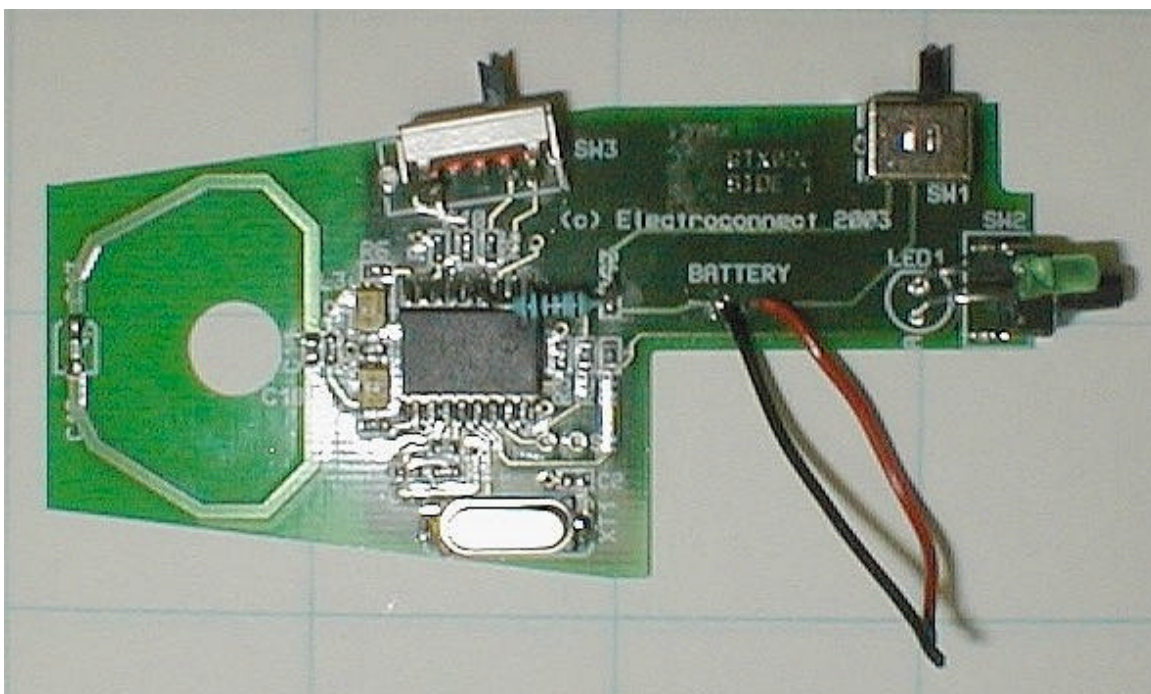
Top View of Board
