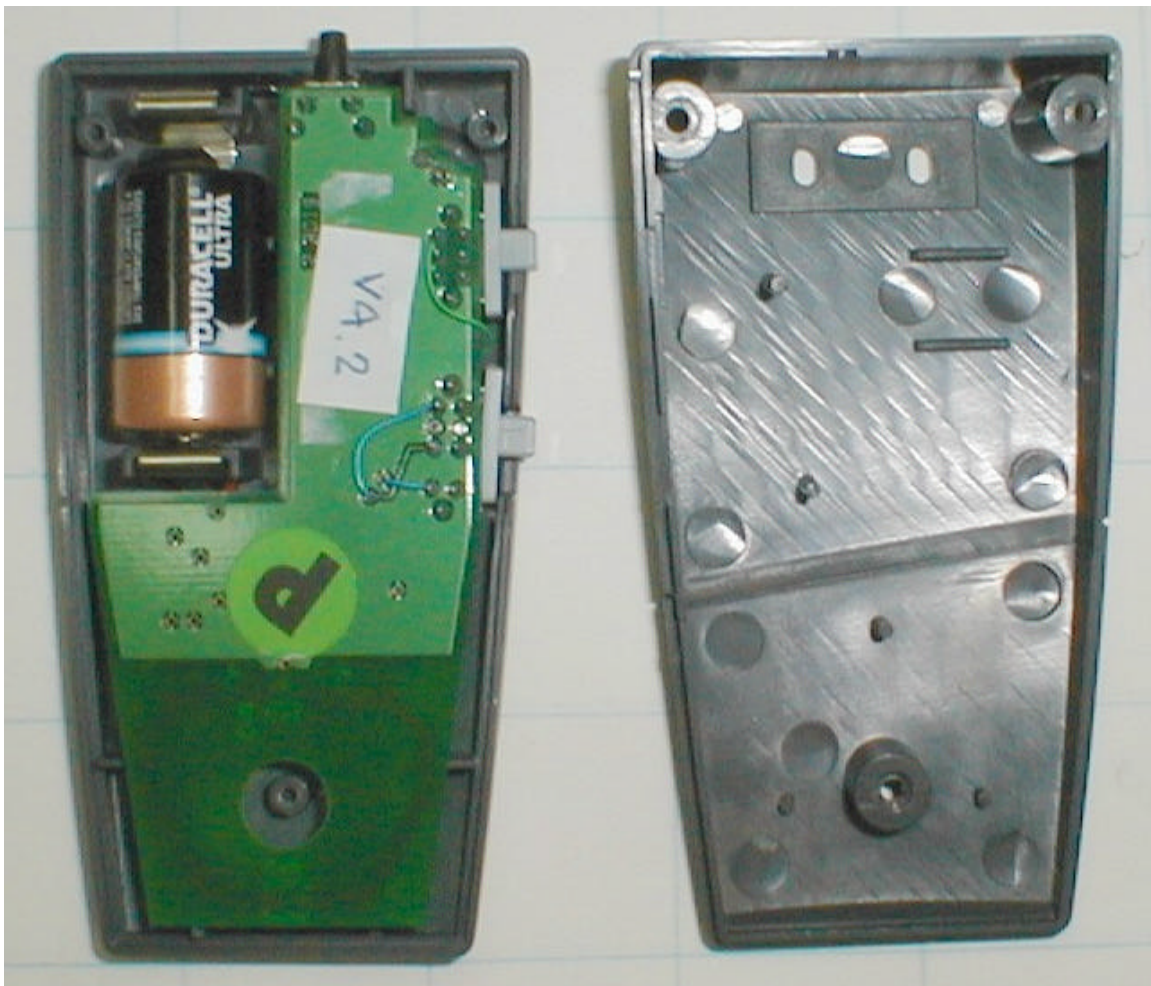
View of Open Housing
