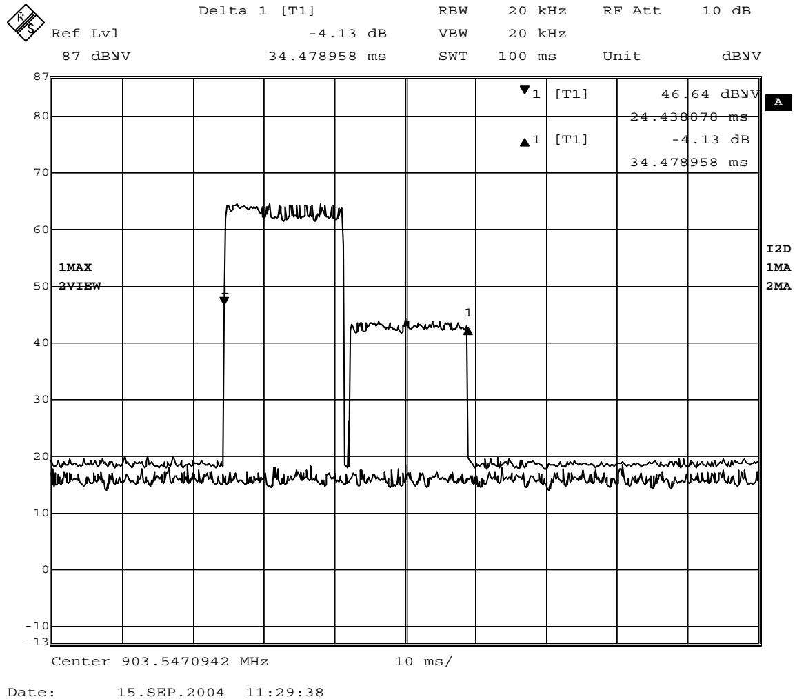
Figure 6 Digital transmissions
