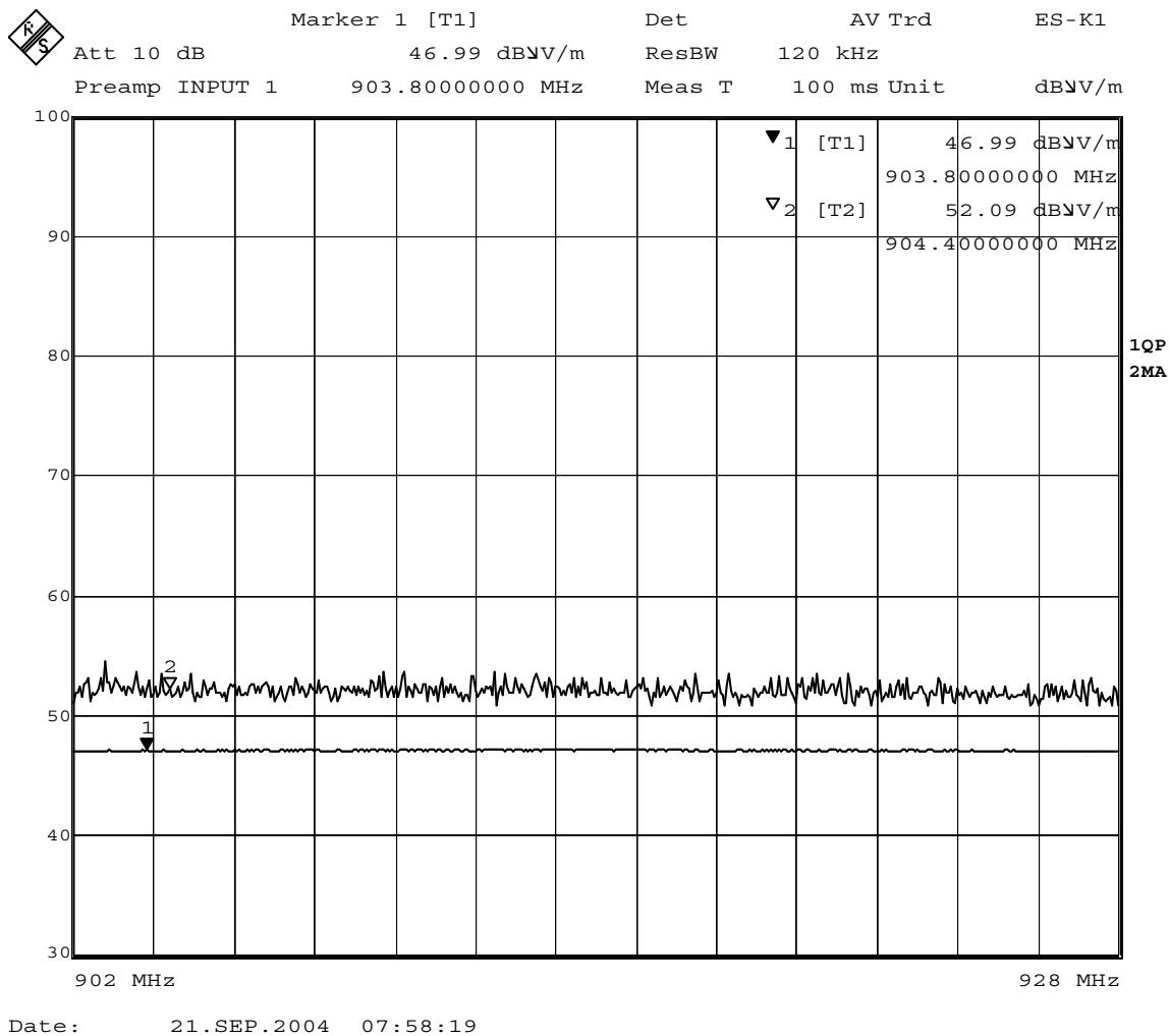
Figure 9 15-minutes of observation. Trace 2 is PEAK, Trace 1 is QUASI-PEAK, both traces set to MAX-HOLD
