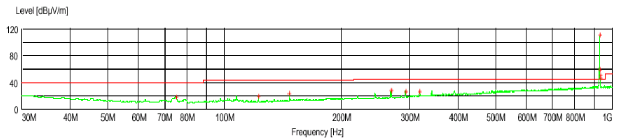
Figure 17 DTS-mode, Channel 31, 15dBm setting
