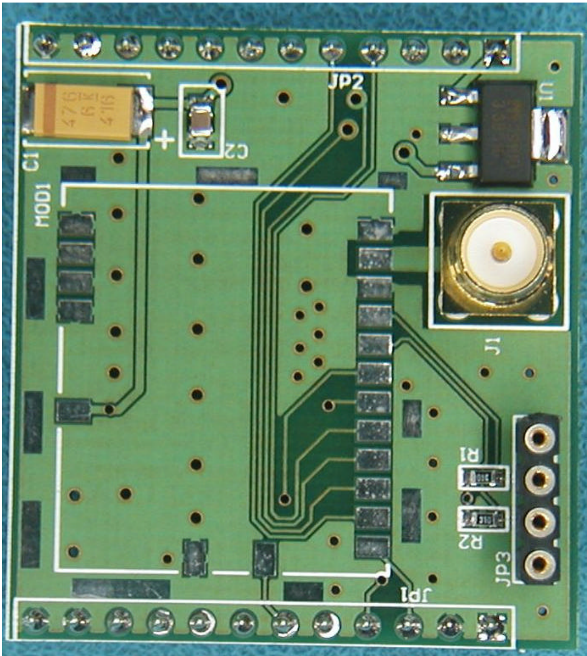
Figure 3 Module without RF daughter board
