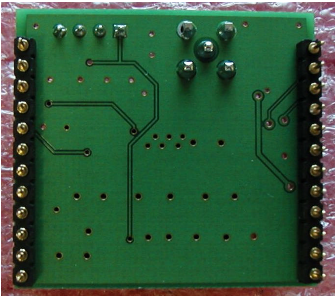
Figure 5 Bottom of module, no label
