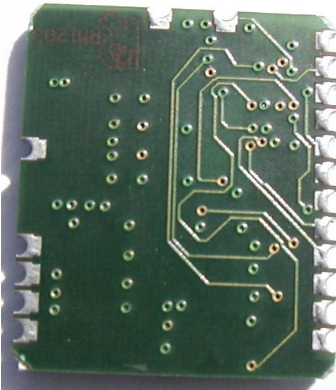
Figure 7 Bottom of RF daughter board
