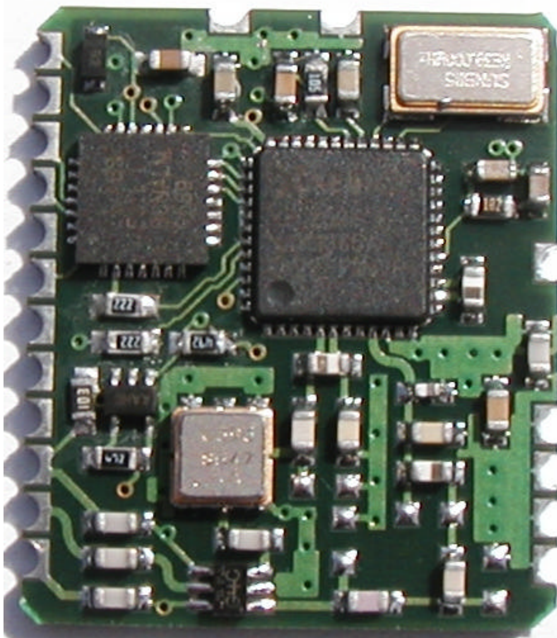
Figure 6 RF daughter board
