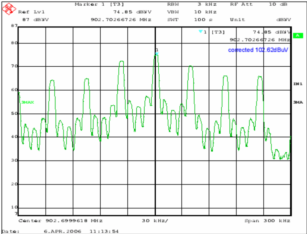
Figure 16 - Power Spectral Density, Channel 0, Radiated
