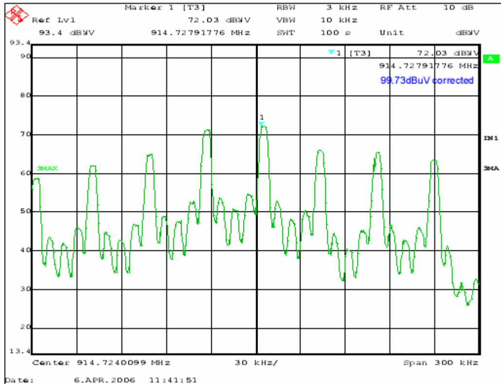
Figure 17 - Power Spectral Density, Channel 16, Radiated
