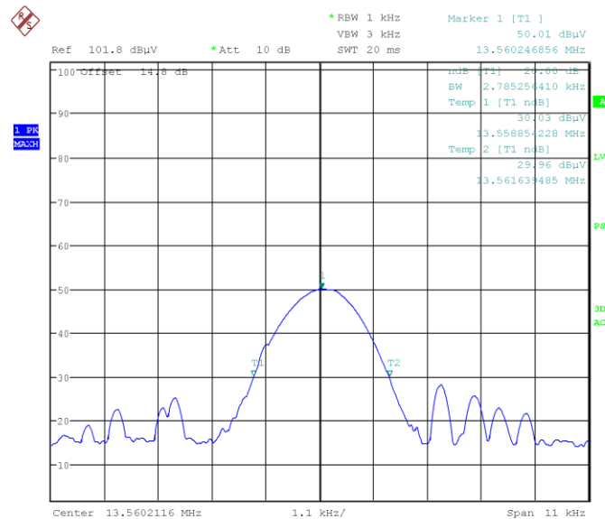
Figure 7.5-2: 20 dB bandwidth
