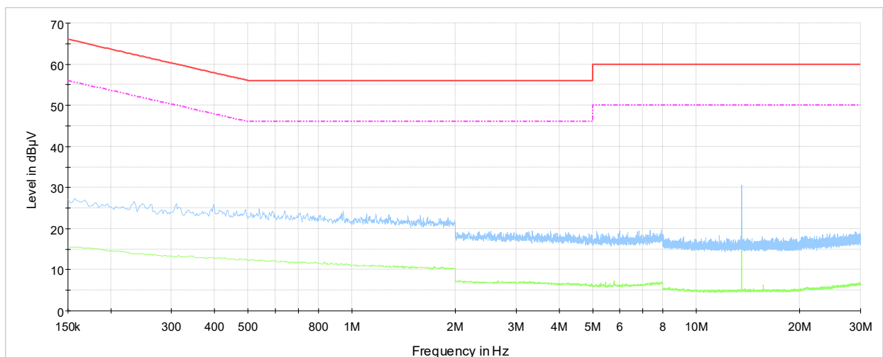
Plot 7.4-1: Conducted emissions on phase line
