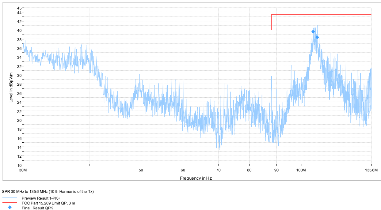
Figure 7.7-2: Field strength of spurious emissions above 30 MHz
