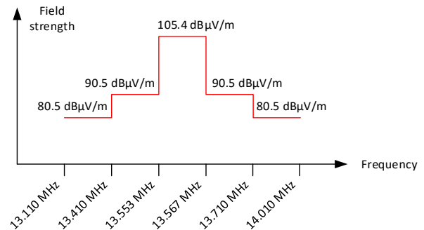
Figure 7.6-2: In-band spurious emissions limit at 3 m
