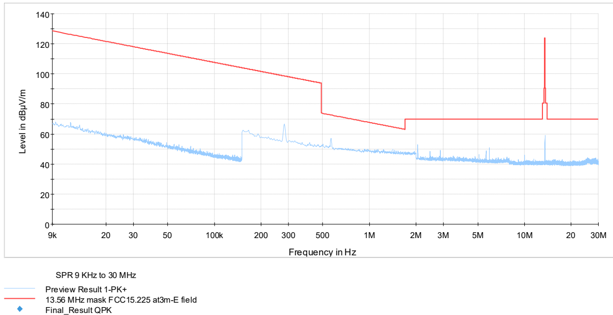
Figure 7.7-1: Field strength of spurious emissions below 30 MHz
