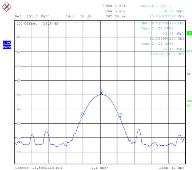
Figure 7.5-1: 99% bandwidth
