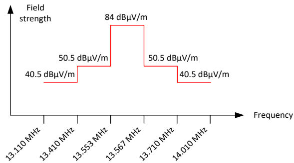
Figure 7.6-1: In-band spurious emissions limit at 30 m
