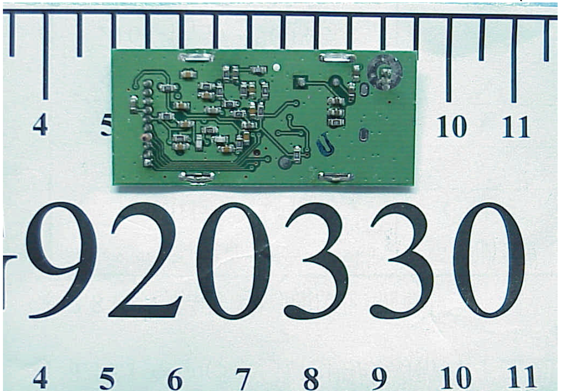
Photo 12 Camera/Transmitter- TX Module (Foil Side)
