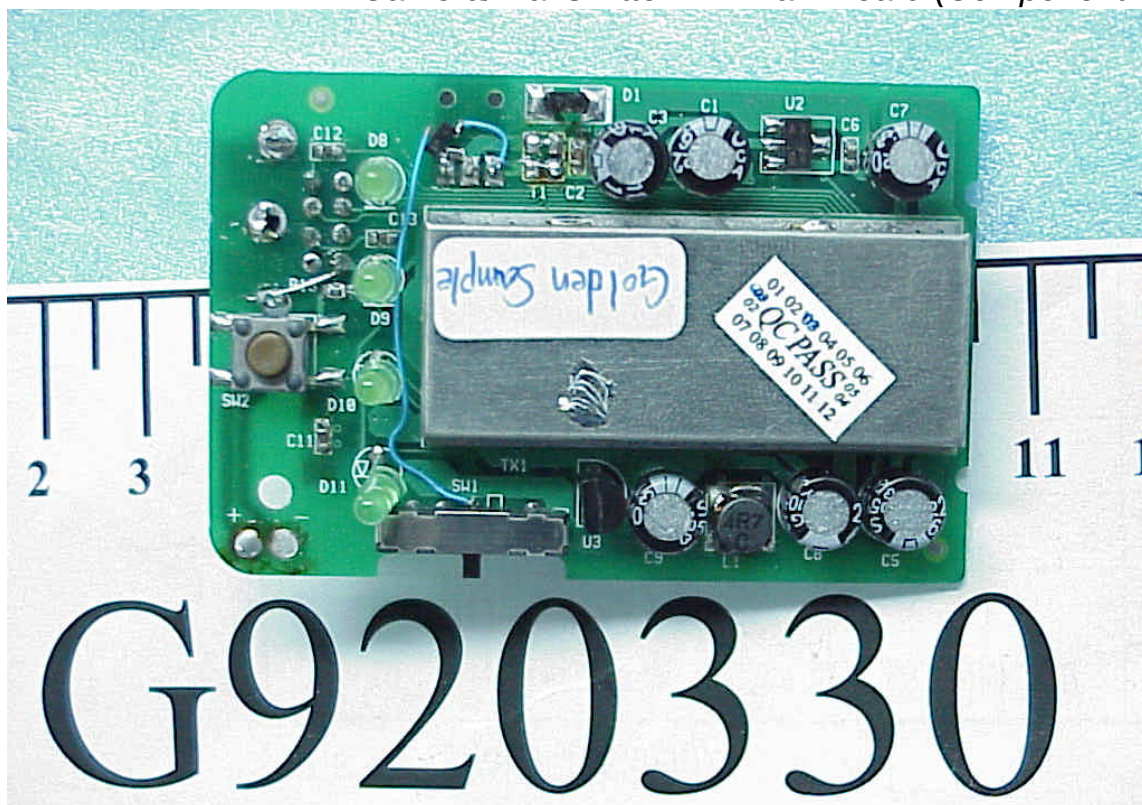
Camera/Transmitter- TX Main Board (Component Side)
