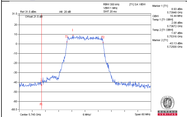
802.11ac(VHT20)_Chain0 / CH149
