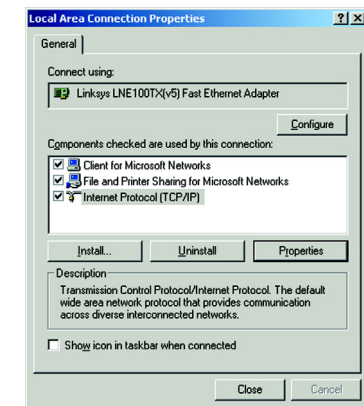
Figure 5-4: TCP/IP
