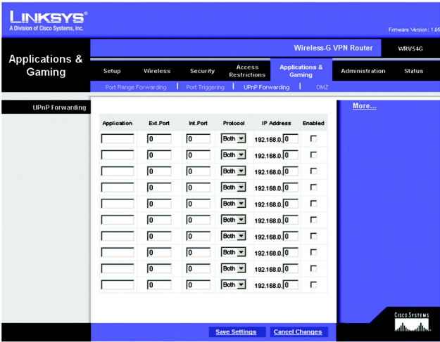
Figure 6-28: UPnP Forwarding
