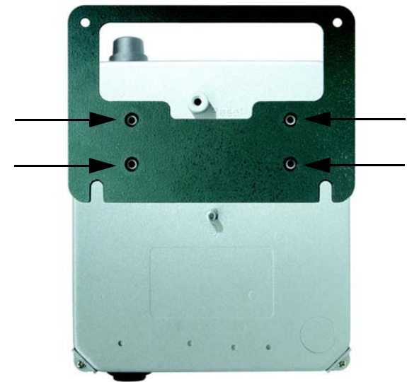
Figure 4-2: Attach the Mounting Plate
