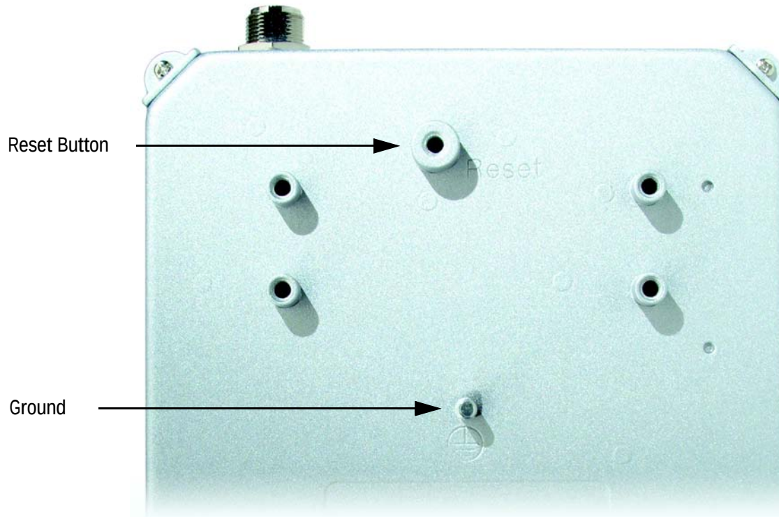
Figure 3-4: Reset Button
