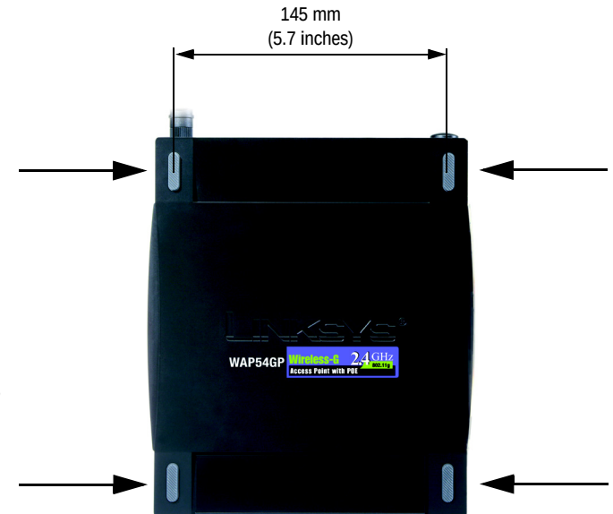
Figure 4-4: The Access Point's Wall-Mount Slots
