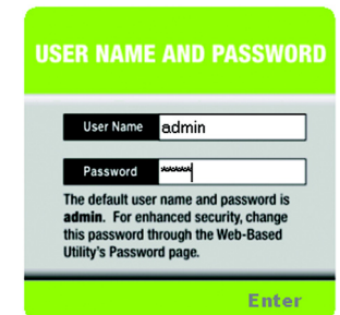
Figure 5-7: Login Screen
