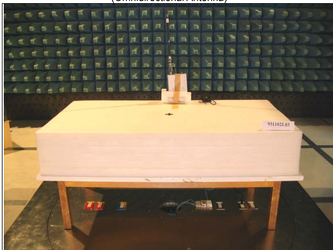
(Omnidirectional Antenna)
