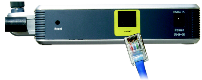
Figure 4-1: Connect the Ethernet Network Cable
