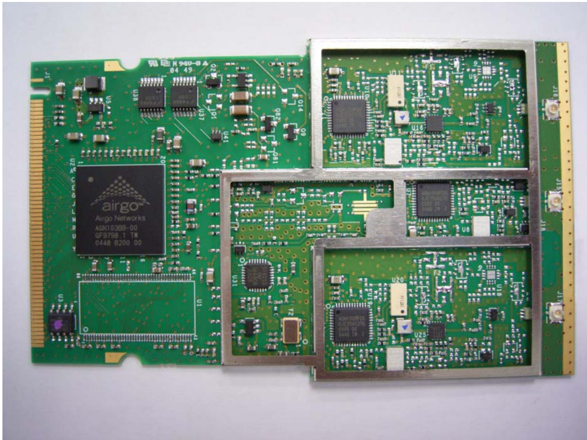
Airgo RF module photo (2048x1536x16M jpeg)
