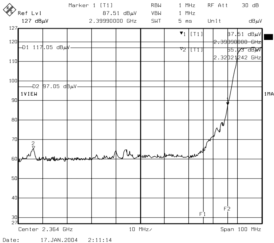
FRONT (Peak)
