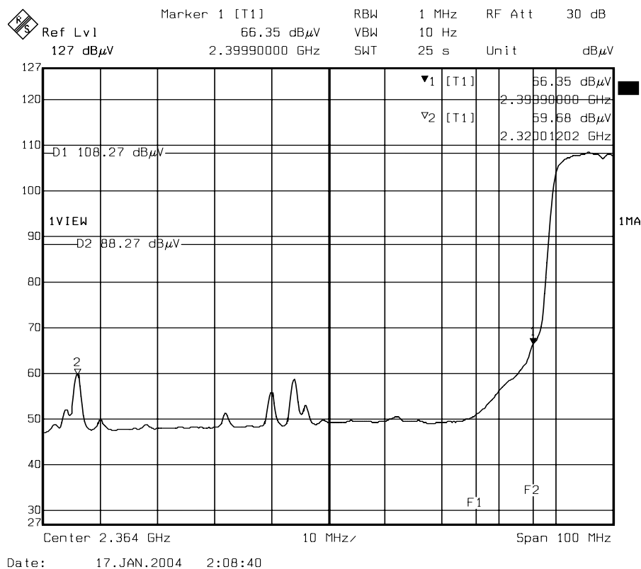
FRONT (AVG)
