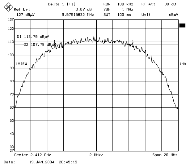
Channel 1
