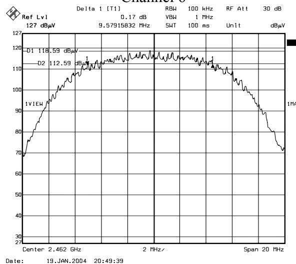
Channel 11
