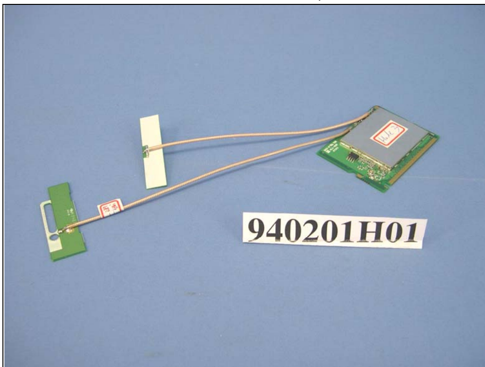
EUT with PIFA antenna and PCB Dipole antenna
